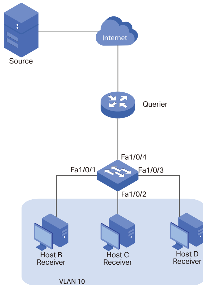
Figure 4-17 Network Topology for Multicast Filtering
