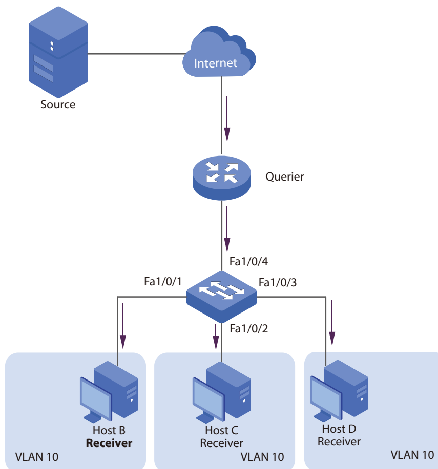
Figure 4-1 Network Topology for Basic IGMP Snooping
