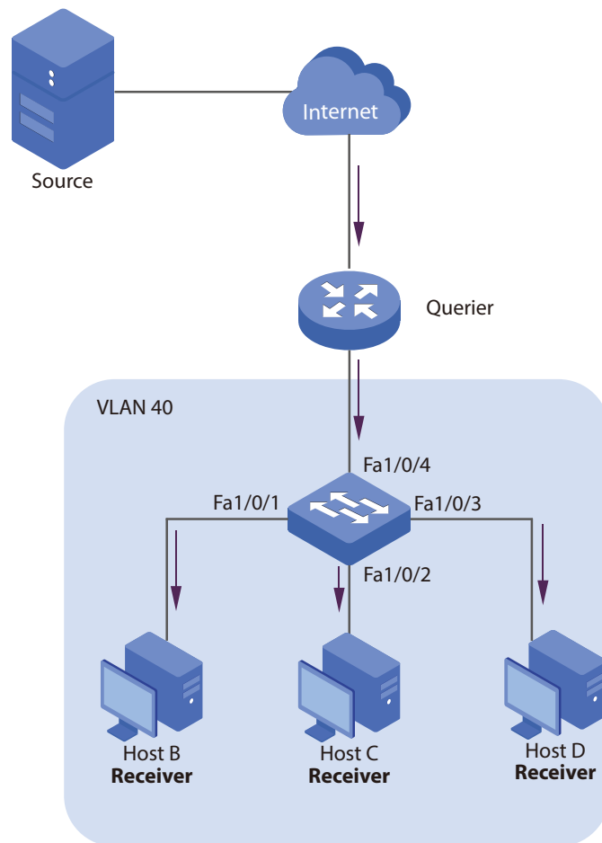
Figure 4-7 Network Topology for Multicast VLAN
