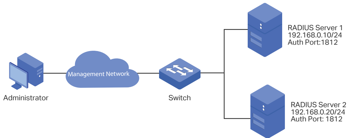
Figure 8-16 Network Topology
