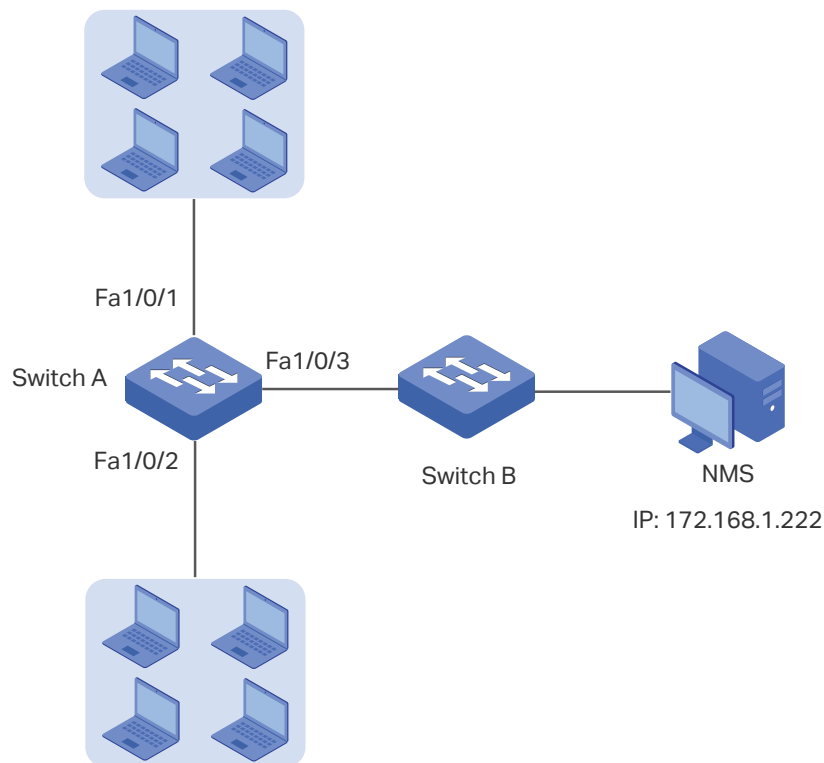
Figure 6-1 Network Topology
