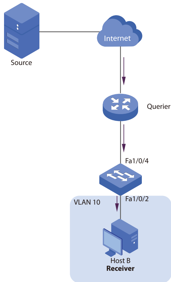
Figure 4-13 Network Topology for Unknow Multicast and Fast Leave
