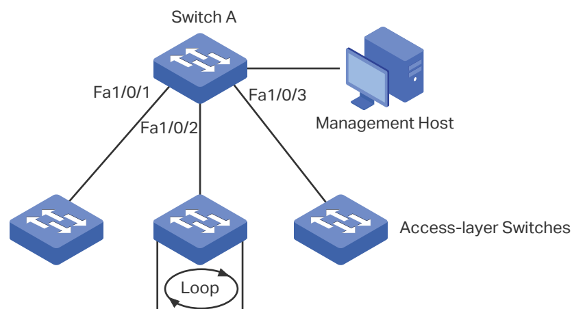
Figure 7-8 Network Topology
