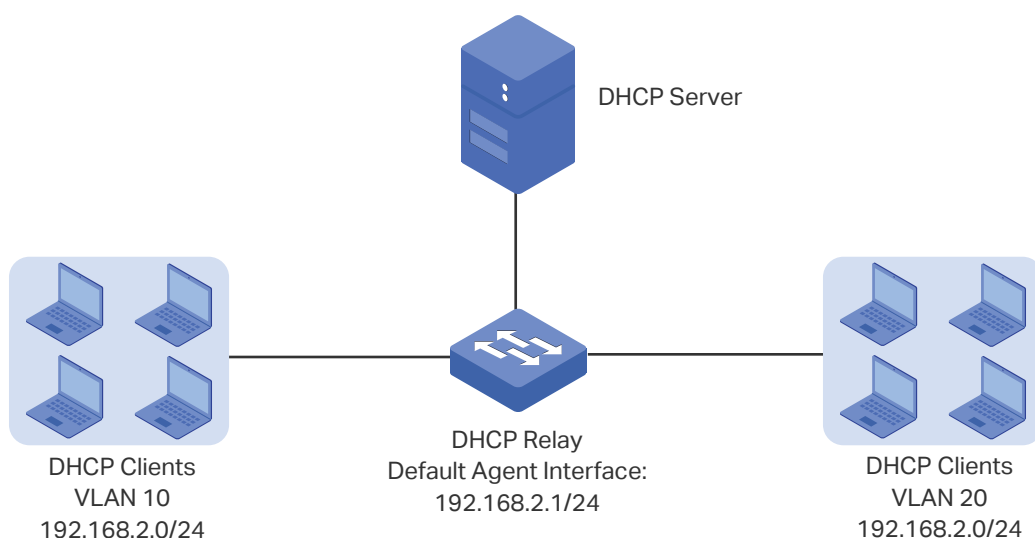
Figure 1-3 Application Scenario of DHCP VLAN Relay
