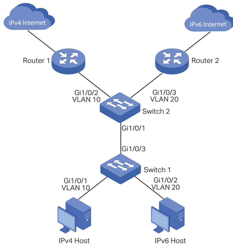
Figure 3-1 Network Topology
