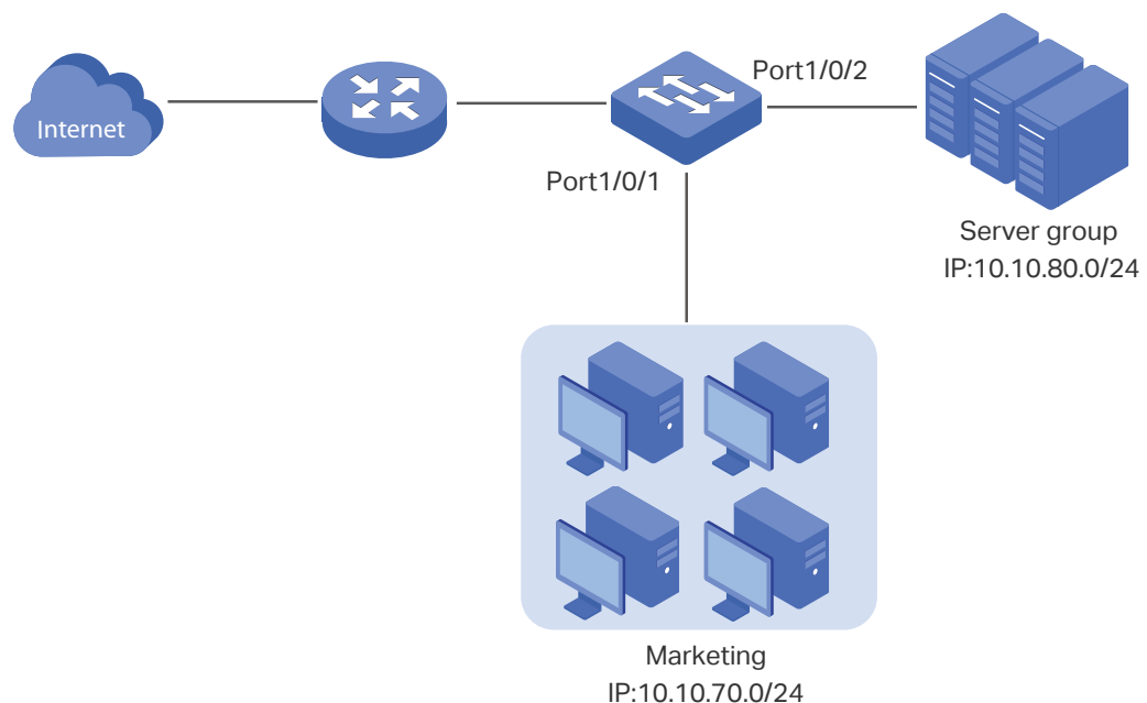
Figure 3-1 Network Topology
