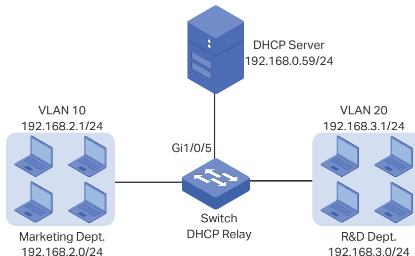
Figure 4-1 Network Topology for DHCP Relay
