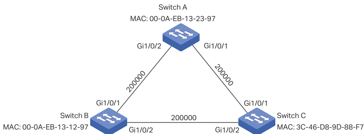
Figure 5-1 Network Topology
