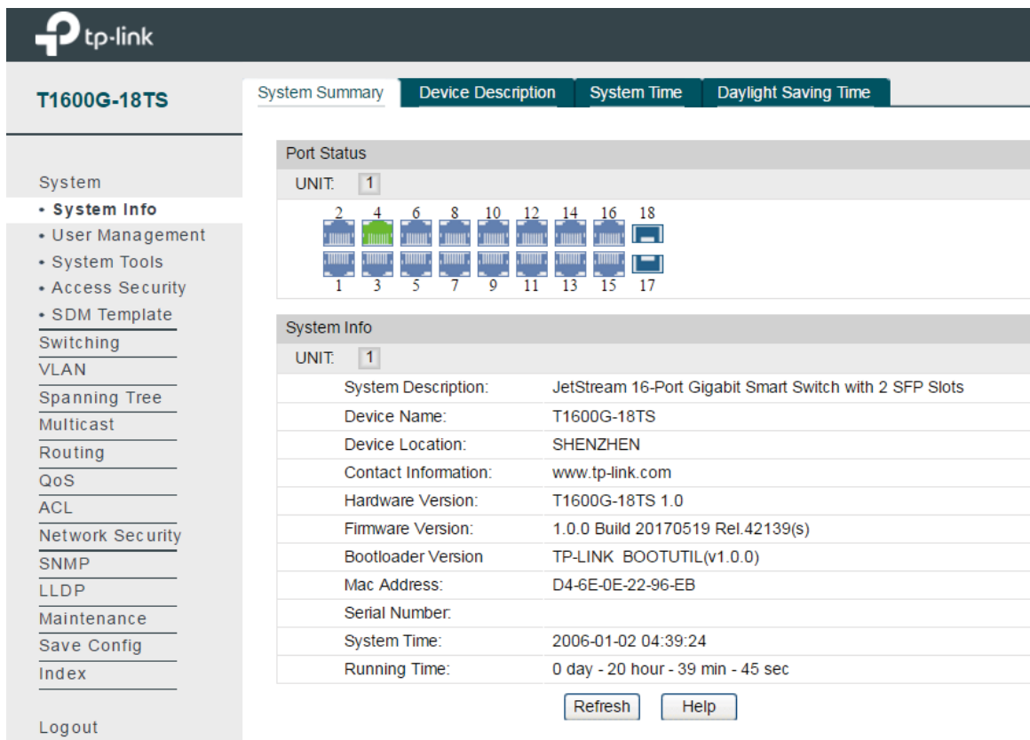
Figure 2-3 Web interface
