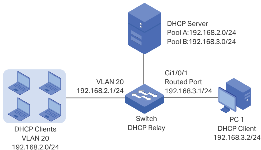
Figure 1-2 Application Scenario of DHCP Interface Relay
