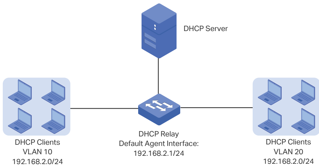
Figure 1-3 Application Scenario of DHCP VLAN Relay
