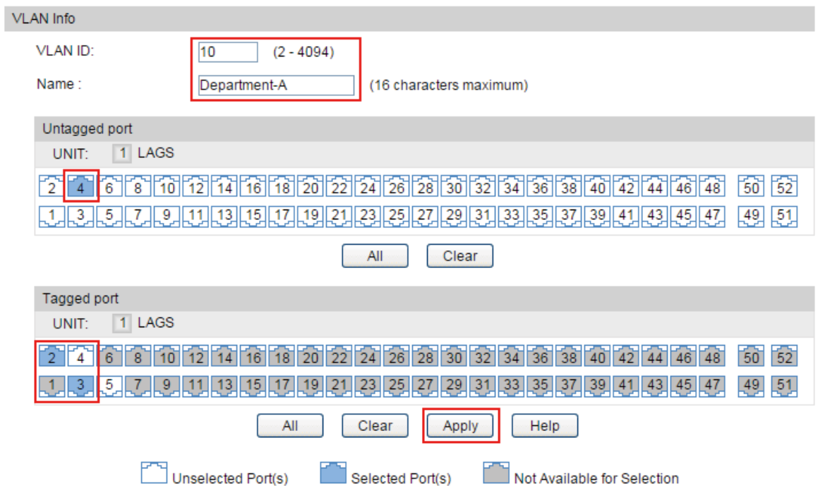
Figure 3-6 VLAN 10 Configuration
