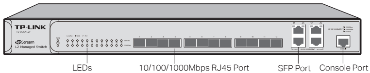
Figure 1-1 Front Panel of TL-SG5412F
