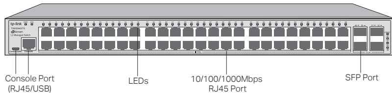
Figure 1-7 Front Panel of T2600G-52TS
