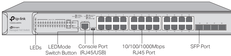
Figure 1-8 Front Panel of T2600G-28MPS
