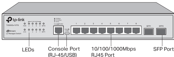
Figure 1-2 Front Panel of TT2500G-10TS
