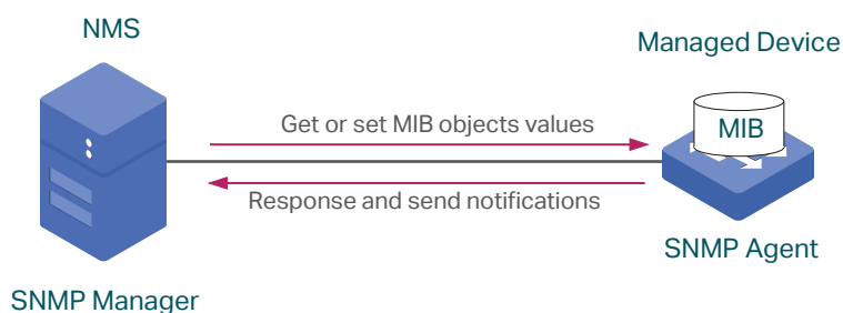
Figure 1-1 SNMP System
