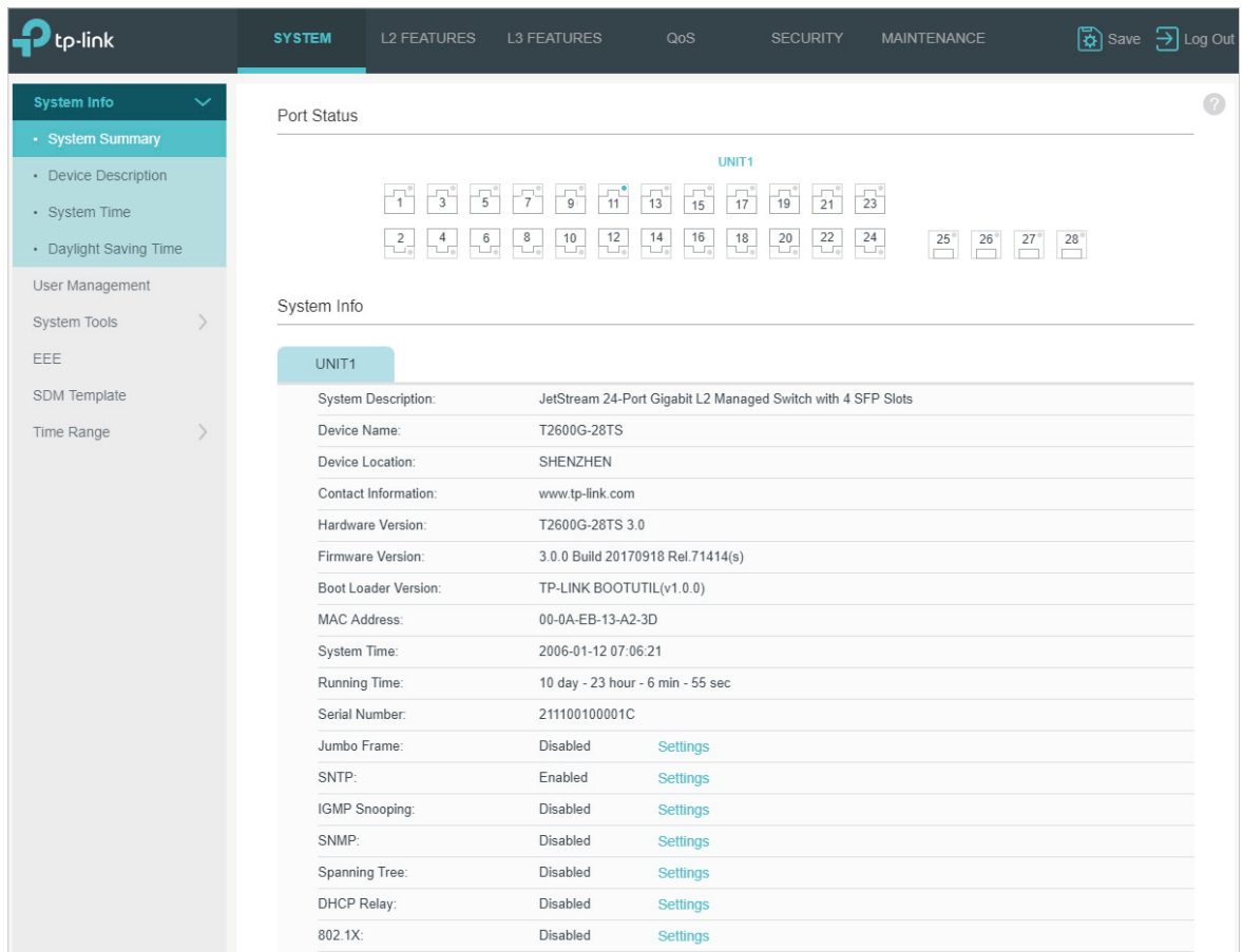
Figure 2-3 Web Interface
