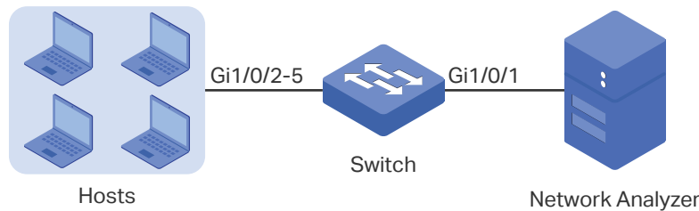
Figure 2-1 Network Topology
