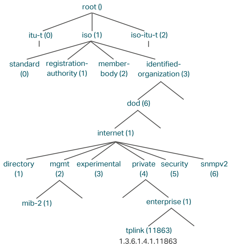
Figure 1-2 MIB Tree
