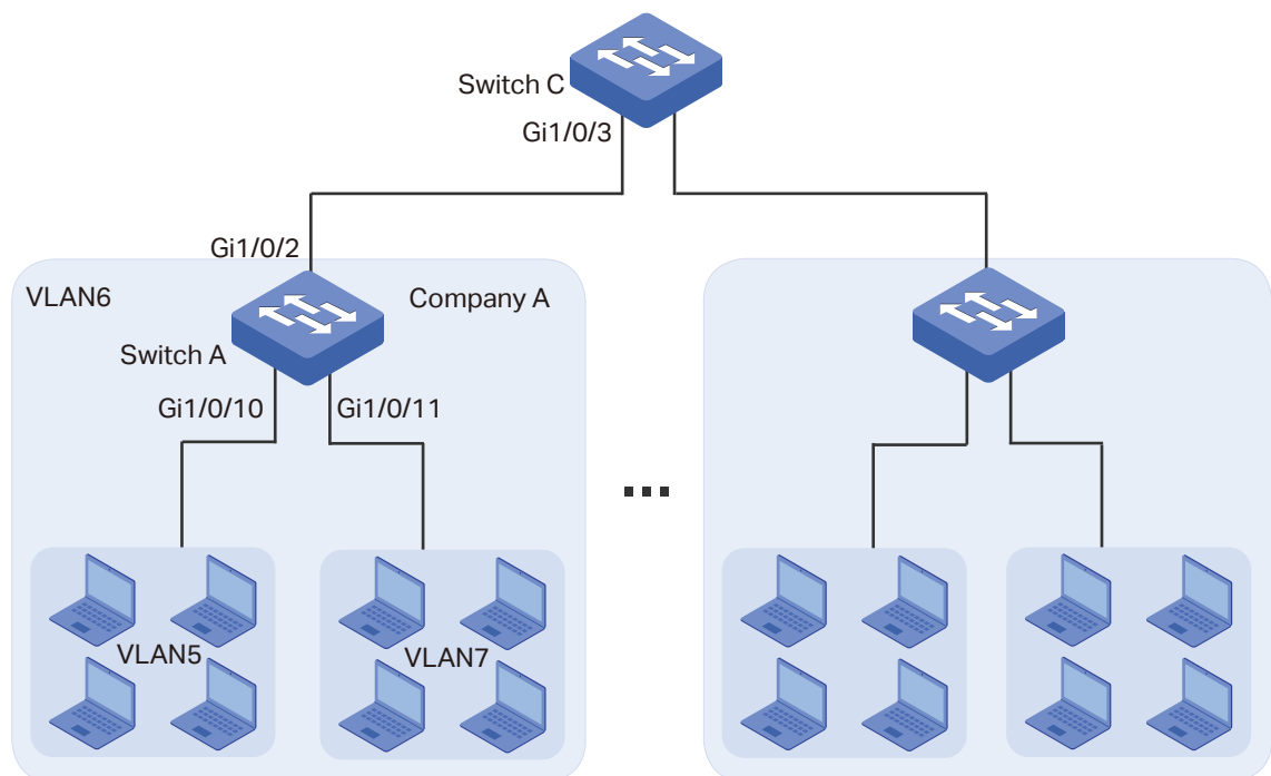
Figure 3-1 Network Topology
