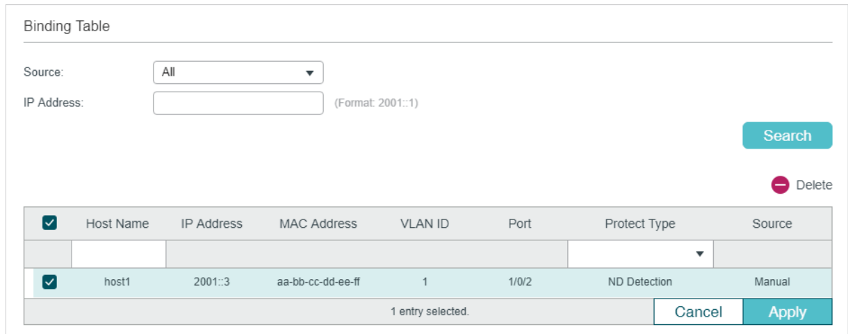
Figure 2-4 Binding Table
