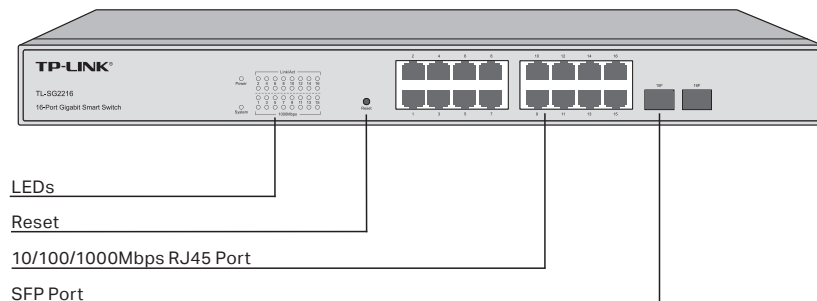
Figure 1-1 Front Panel of TL-SG2216
