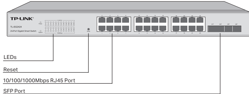
Figure 1-2 Front Panel of TL-SG2424
