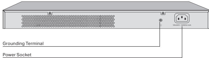
Figure 1-5 Rear Panel
