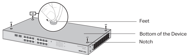
Figure 2-1 Desktop Installation
