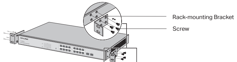
Figure 2-2 Bracket Installation
