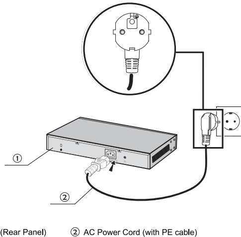
Figure 3-1 Connecting to the Ground
