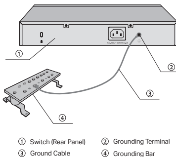
Figure 3-2 Connecting to the Grounding Bar
