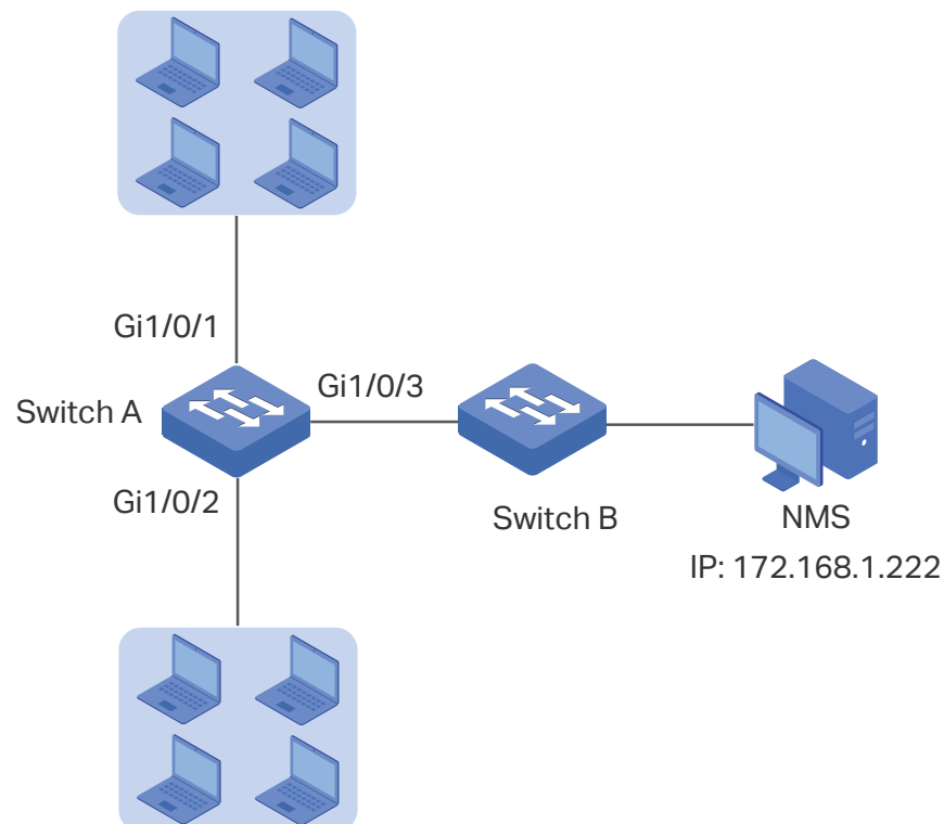
Figure 6-1 Network Topology
