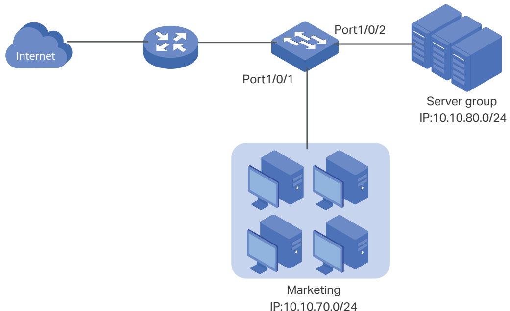
Figure 3-1 Network Topology
