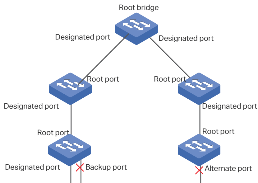
Figure 1-2 STP/RSTP Topology
