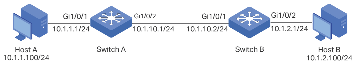
Figure 5-1 Network Topology
