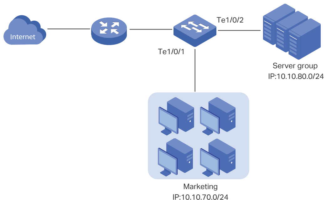
Figure 3-1 Network Topology
