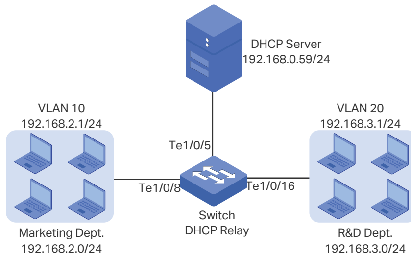
Figure 3-1 Network Topology
