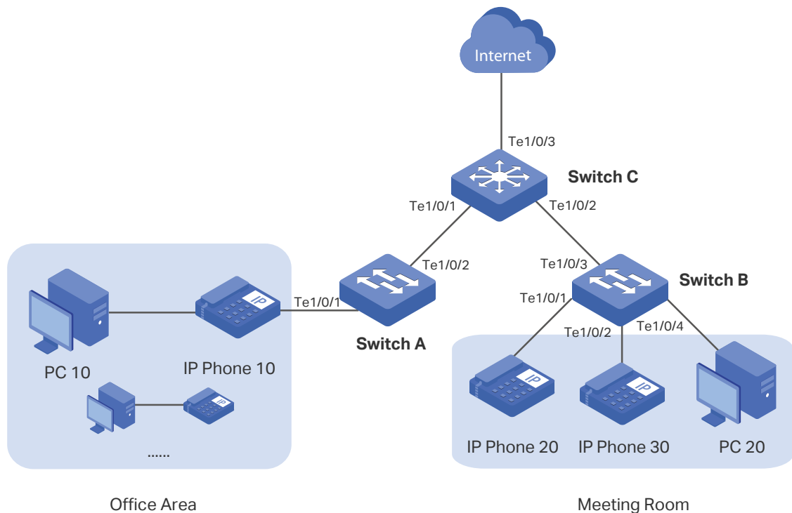
Figure 3-1 Network Topology
