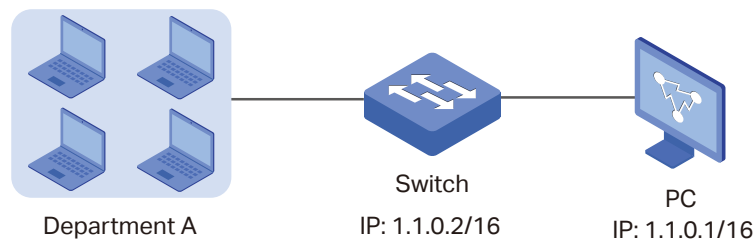
Figure 6-1 Network Topology
