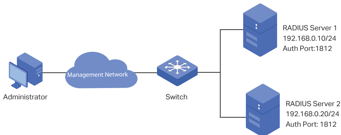
Figure 8-16 Network Topology
