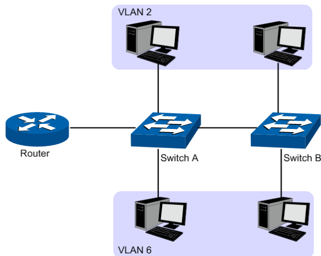
Figure 6-1 VLAN implementation
