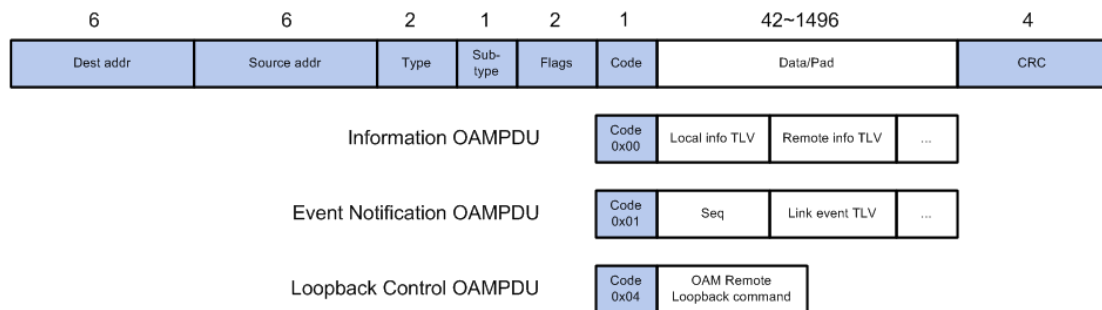
Figure 8-1 OAMPDUs
