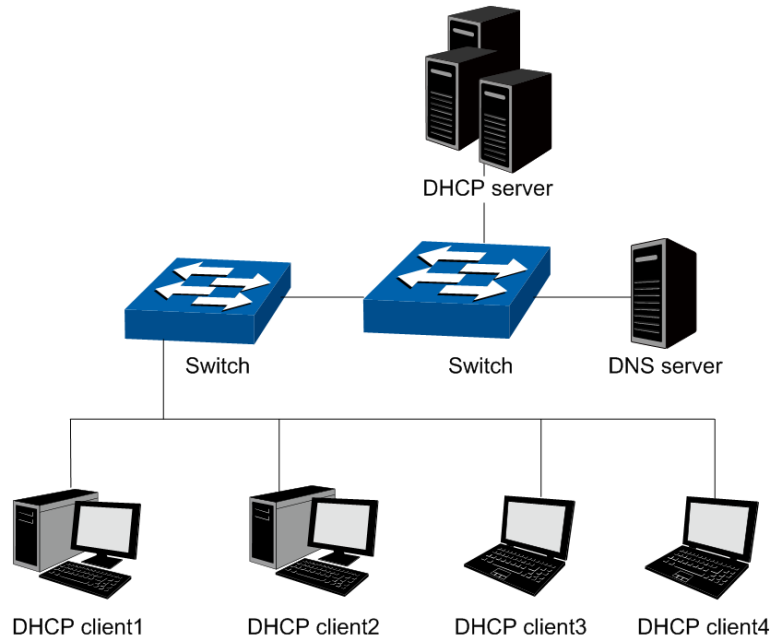
Figure 9-1 DHCP model
