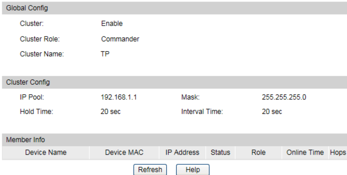
Figure 16-10 Cluster Summary for Commander Switch
