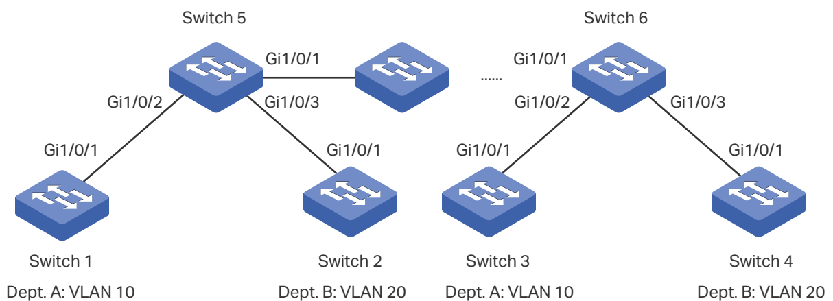
Figure 3-1 Network Topology
