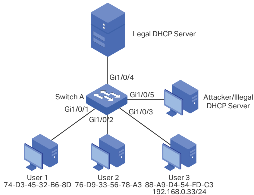
Figure 13-1 Network Topology
