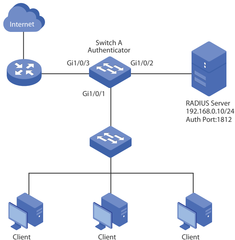
Figure 13-8 Network Topology
