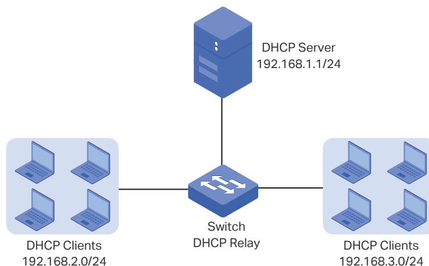
Figure 1-1 Application Scenario of DHCP Interface Relay
