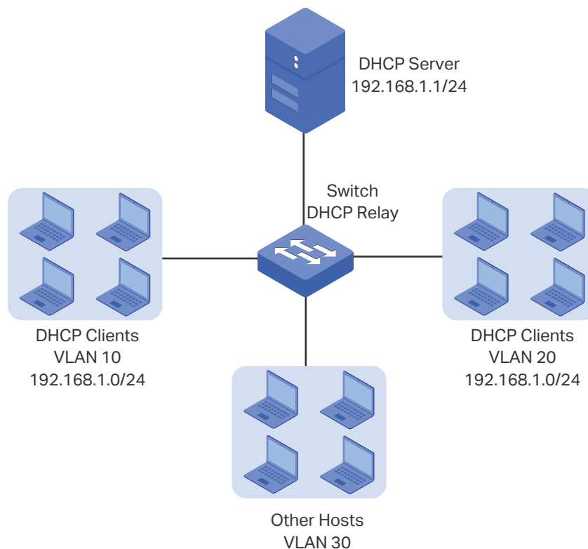
Figure 1-2 Application Scenario of DHCP VLAN Relay
