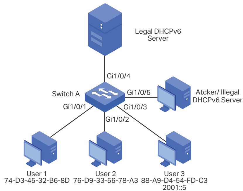
Figure 13-1 Network Topology
