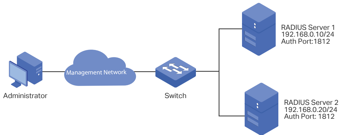
Figure 13-16 Network Topology
