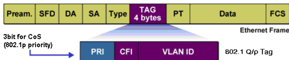
Figure 8-2 802.1Q frame
