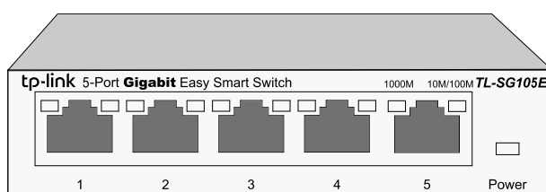
Figure 2-1 Front Panel of TL-SG105E
