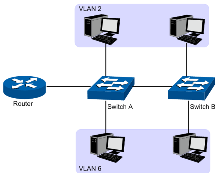
Figure 7-1 VLAN implementation
