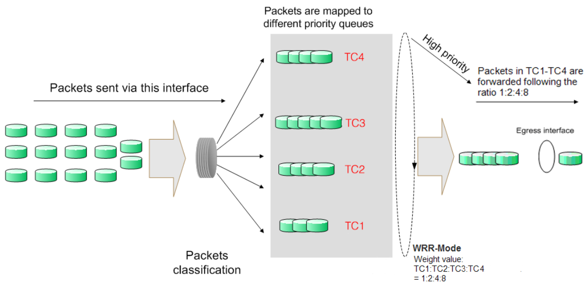
Figure 8-1 QoS function
