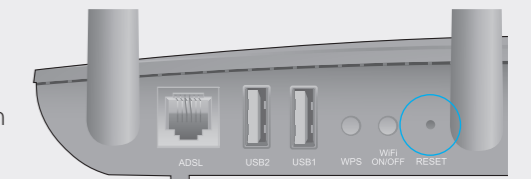
RESET Button Use a Pin to Press & Hold 8 seconds
