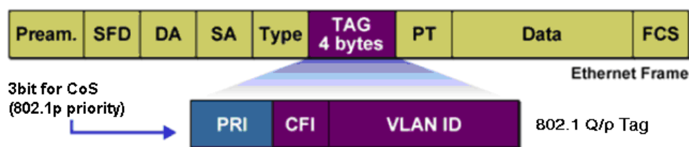
Figure 10-2 802.1Q frame
