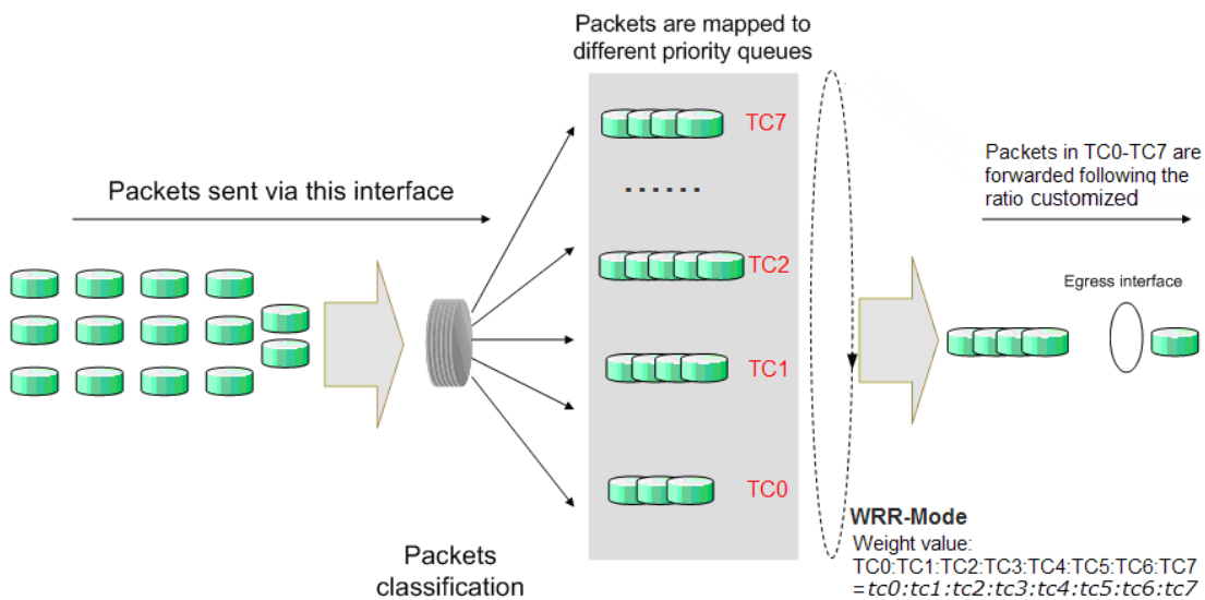
Figure 10-5 WRR-Mode
