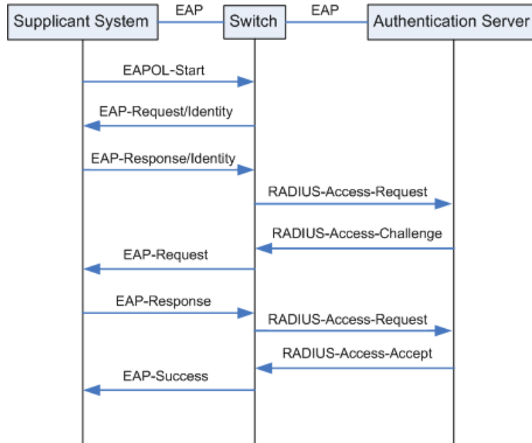
Figure 12-20 EAP-MD5 Authentication Procedure
