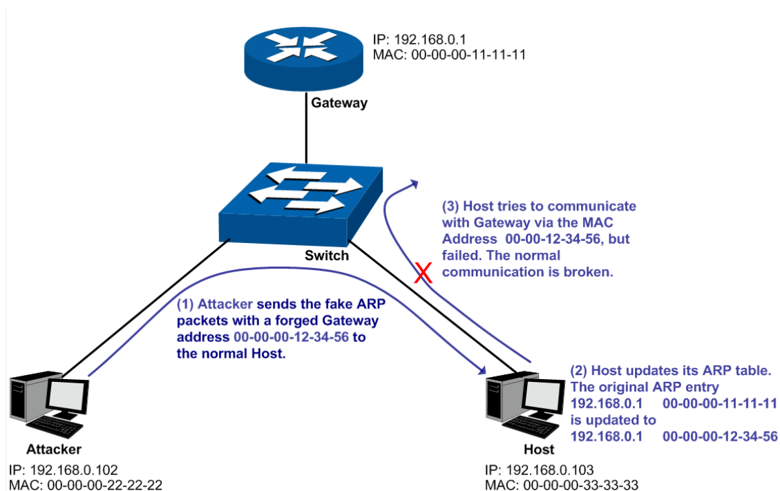
Figure 12-11 ARP Attack - Imitating Gateway
