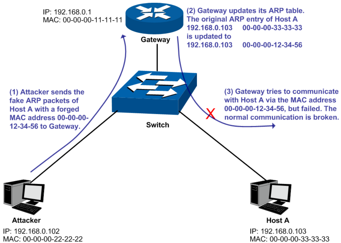
Figure 12-12 ARP Attack – Cheating Gateway
