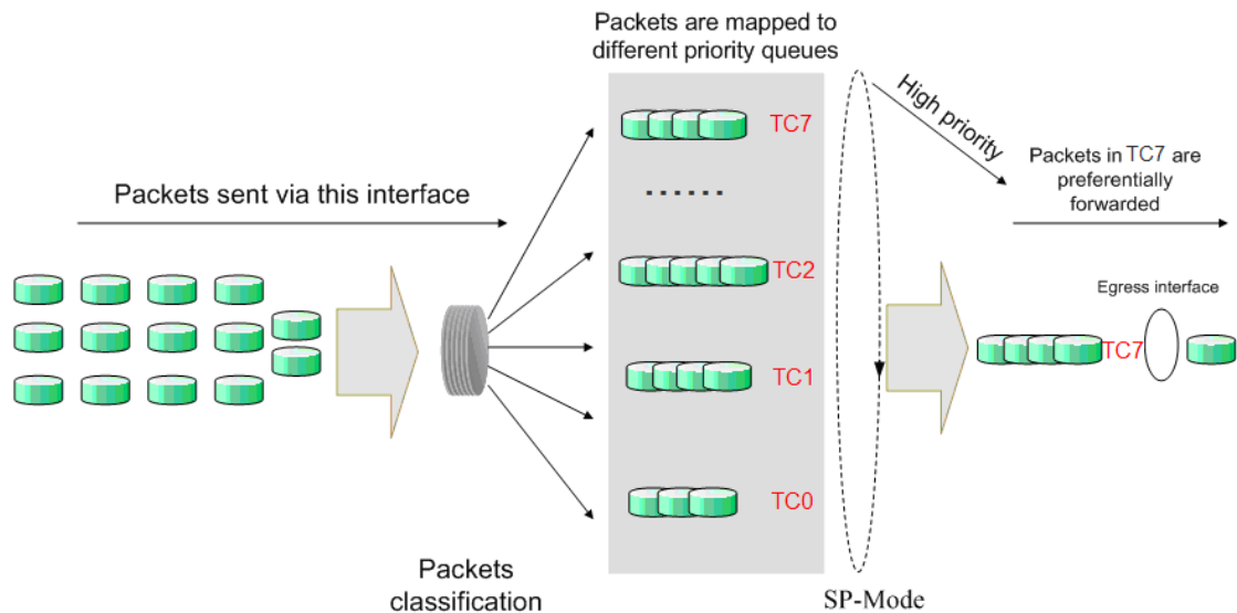
Figure 10-4 SP-Mode
