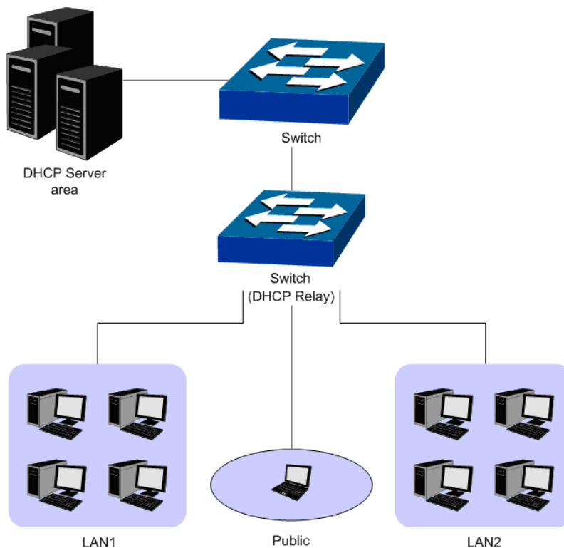
Figure 9-9 DHCP Relay Application
