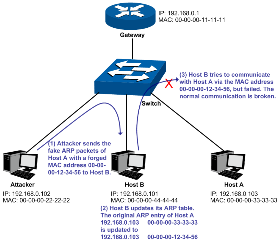
Figure 12-13 ARP Attack – Cheating Terminal Hosts
