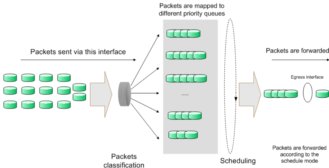
Figure 10-1 QoS function
