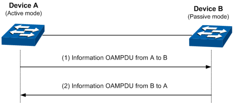
Figure 8-2 OAM Discovery
