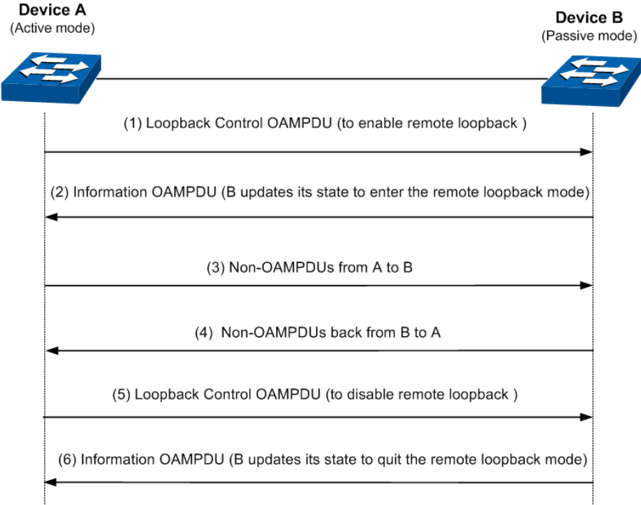
Figure 8-3 Remote Loopback
