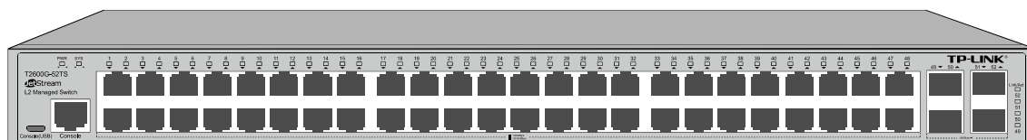
Figure 2-2 Front Panel of T2600G-52TS
