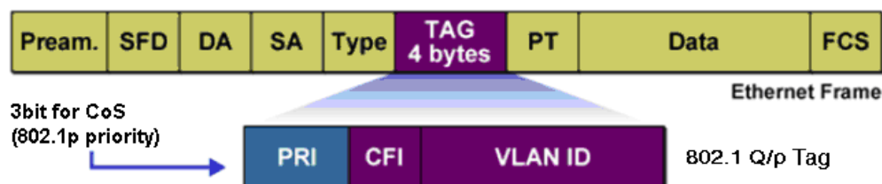
Figure 11-2 802.1Q frame
