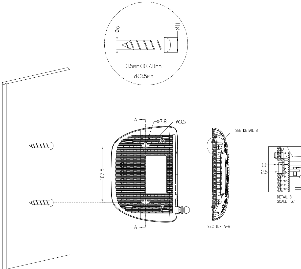
Figure 2-1 Wall-mount Install
