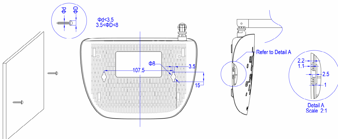
Figure 2-1 Wall-mount Install
