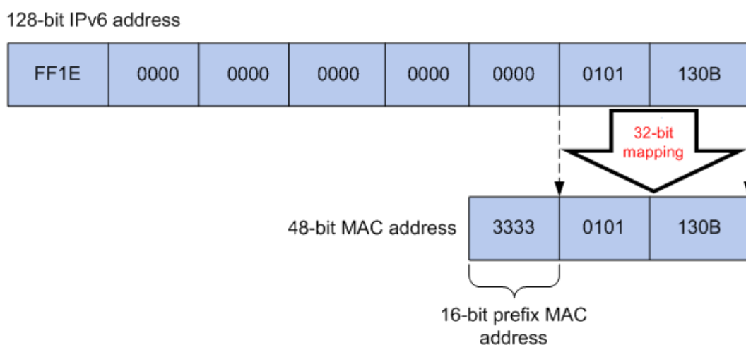
Figure 8-3 Mapping relationship between multicast IPv6 address and multicast IPv6 MAC address
