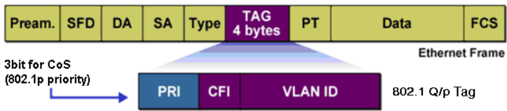
Figure 9-2 802.1Q frame
