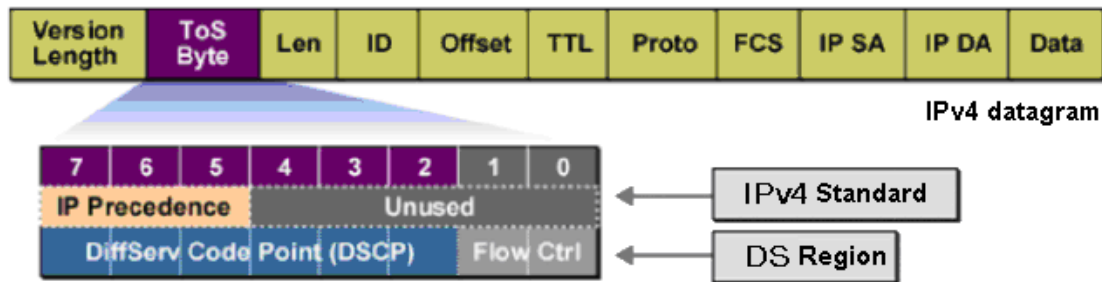
Figure 9-3 IP datagram
