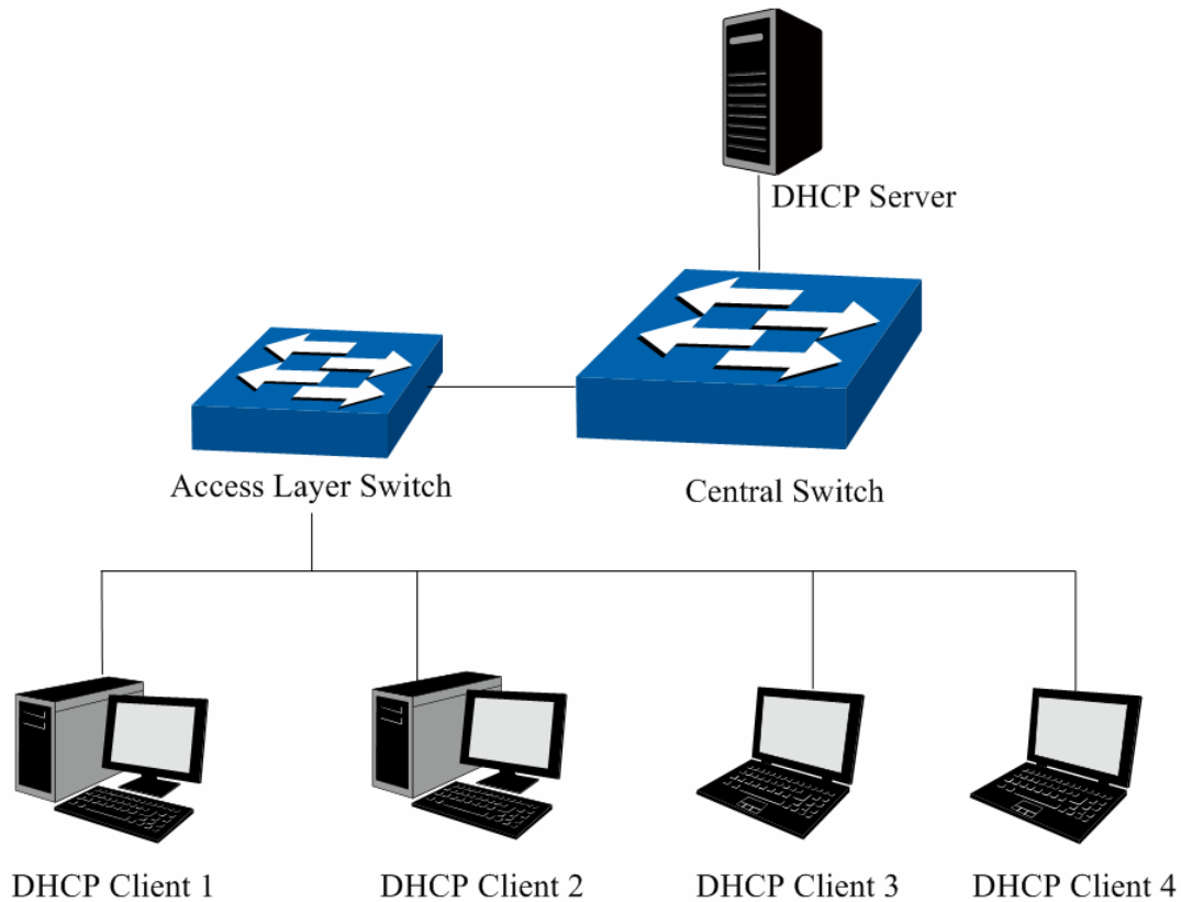
Figure 13-5 Network diagram for DHCP-snooping implementation
