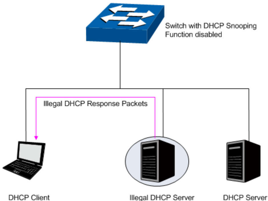
Figure 13-7 DHCP Cheating Attack Implementation Procedure
