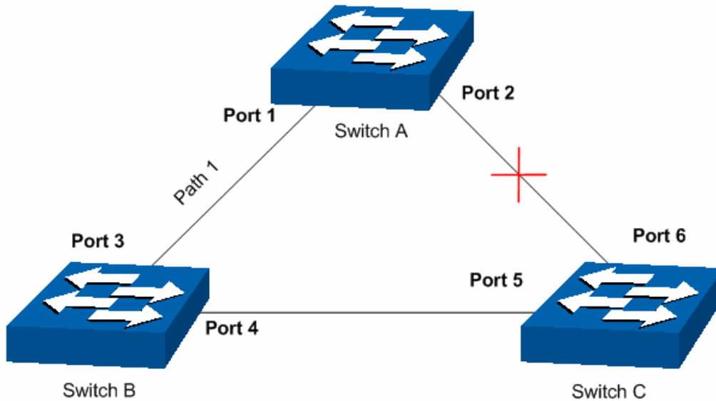
Figure 9-1 Basic STP diagram
