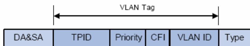
Figure 8-2 Format of VLAN Tag
