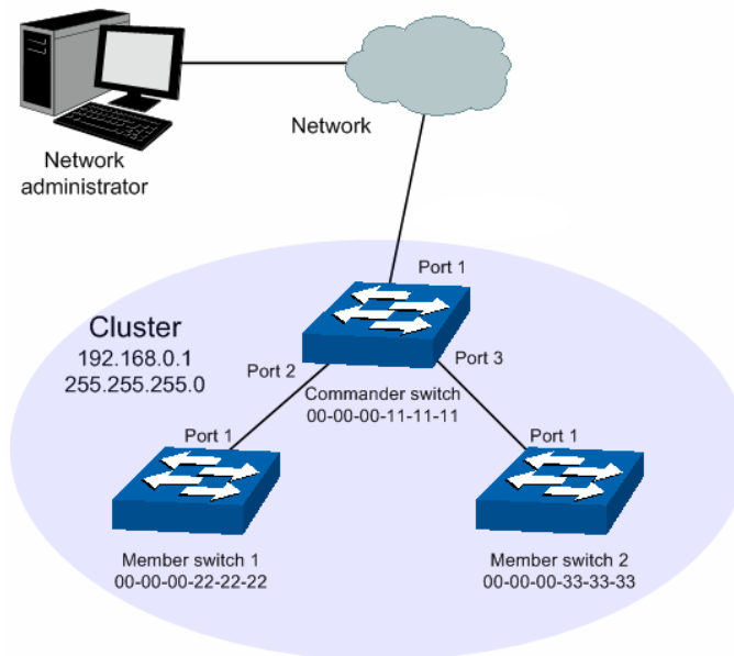
Figure 13-19 Network diagram
