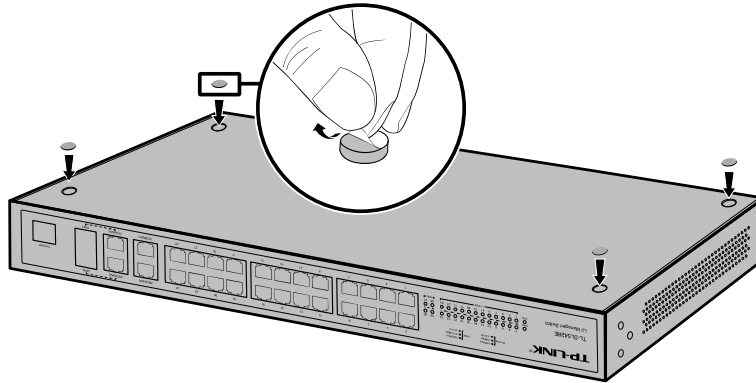
Figure 3-1 Attaching Rubber Feet
