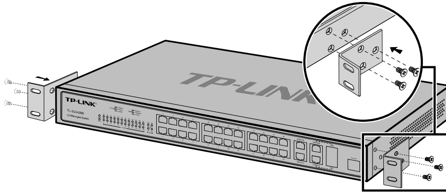
Figure 3-2 Attaching Brackets
