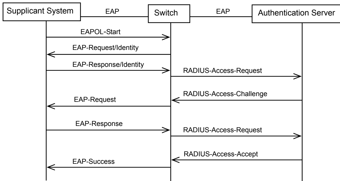
Figure 13-20 EAP-MD5 Authentication Procedure
