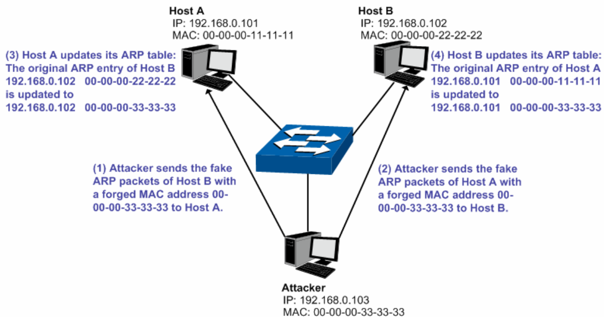
Figure 13-12 Man-In-The-Middle Attack
