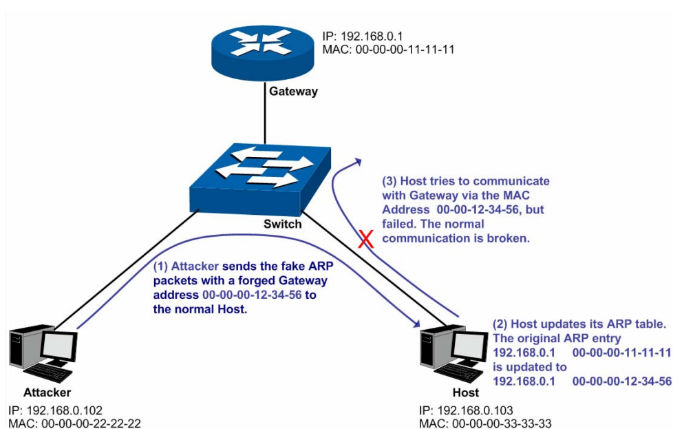
Figure 13-9 ARP Attack - Imitating Gateway
