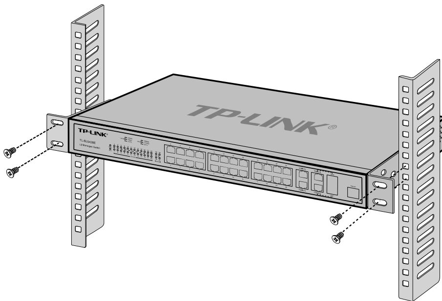
Figure 3-3 Mounting Switch
