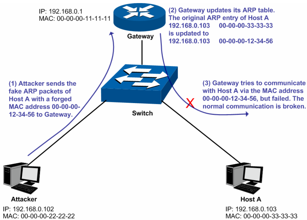
Figure 13-10 ARP Attack – Cheating Gateway
