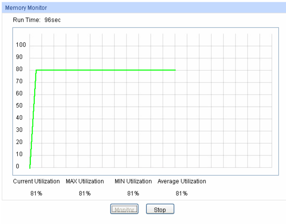
Figure 16-2 Memory Monitor
