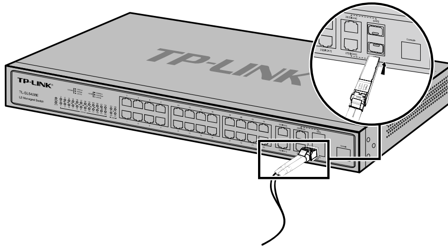
Figure 4-2 Inserting SFP Module
