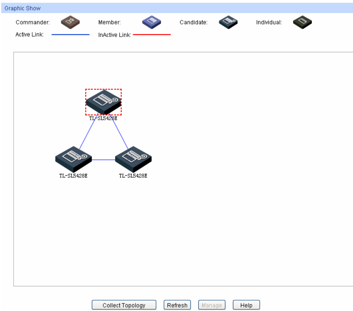
Figure 15-18 Collect Topology
