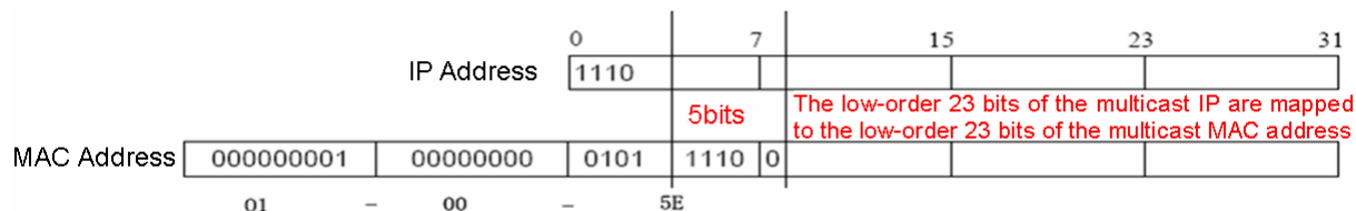
Figure 10-2 Mapping relationship between multicast IP address and multicast MAC address
