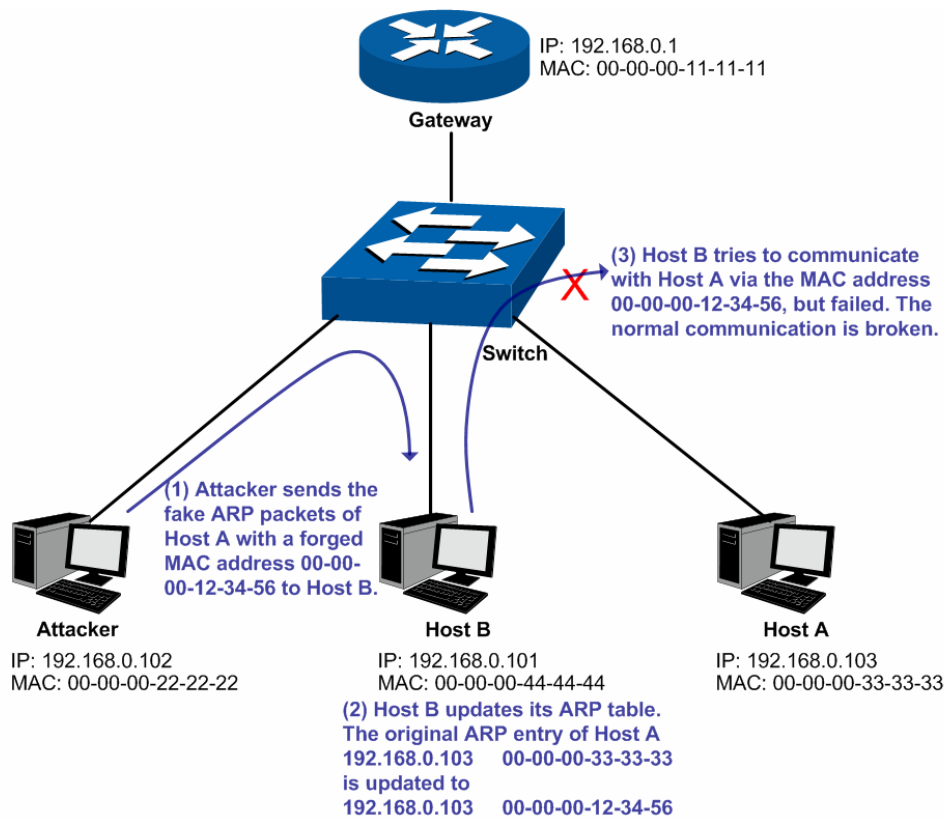
Figure 13-11 ARP Attack – Cheating Terminal Hosts
