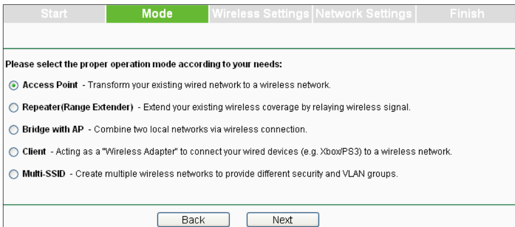
Figure 3-5 Operation Mode
