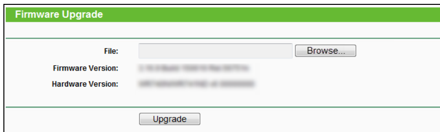
Figure 4-90 Firmware Upgrade
