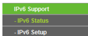
Figure 4-77 IPv6 Support
