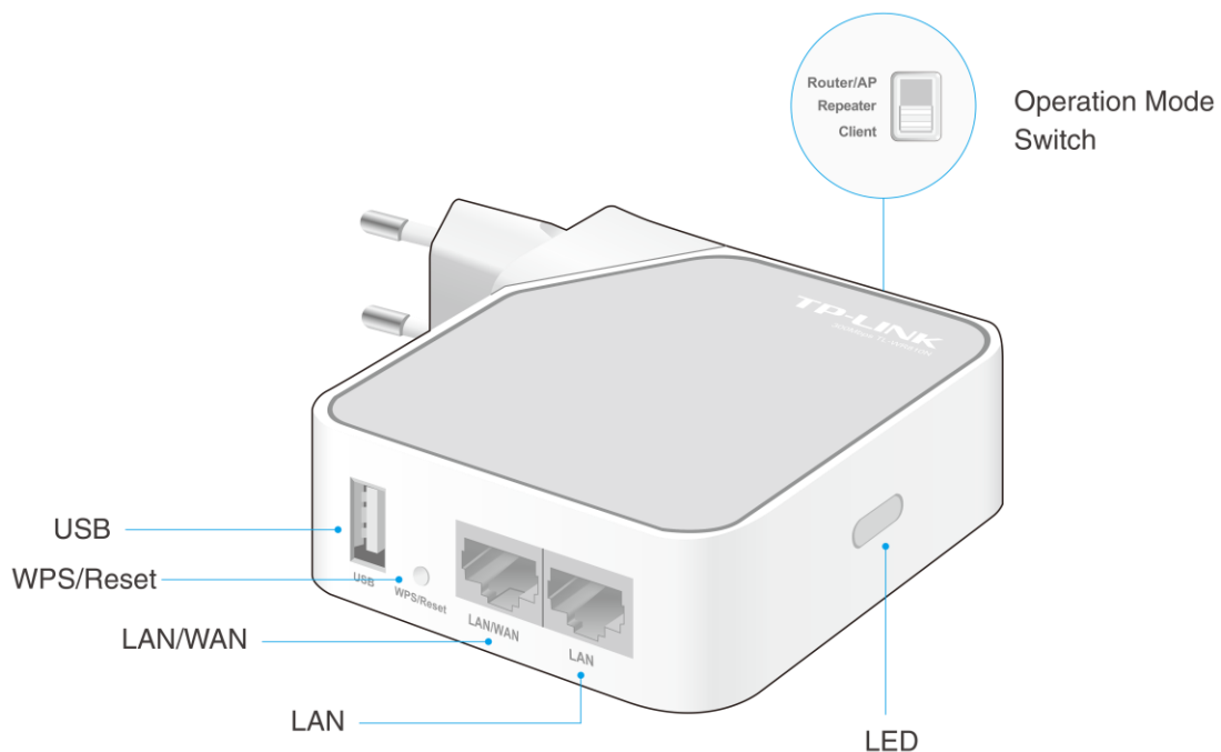
Figure 1-1 TL-WR810N sketch
