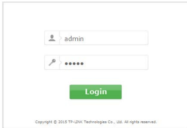
Figure 3-4 Login Windows
