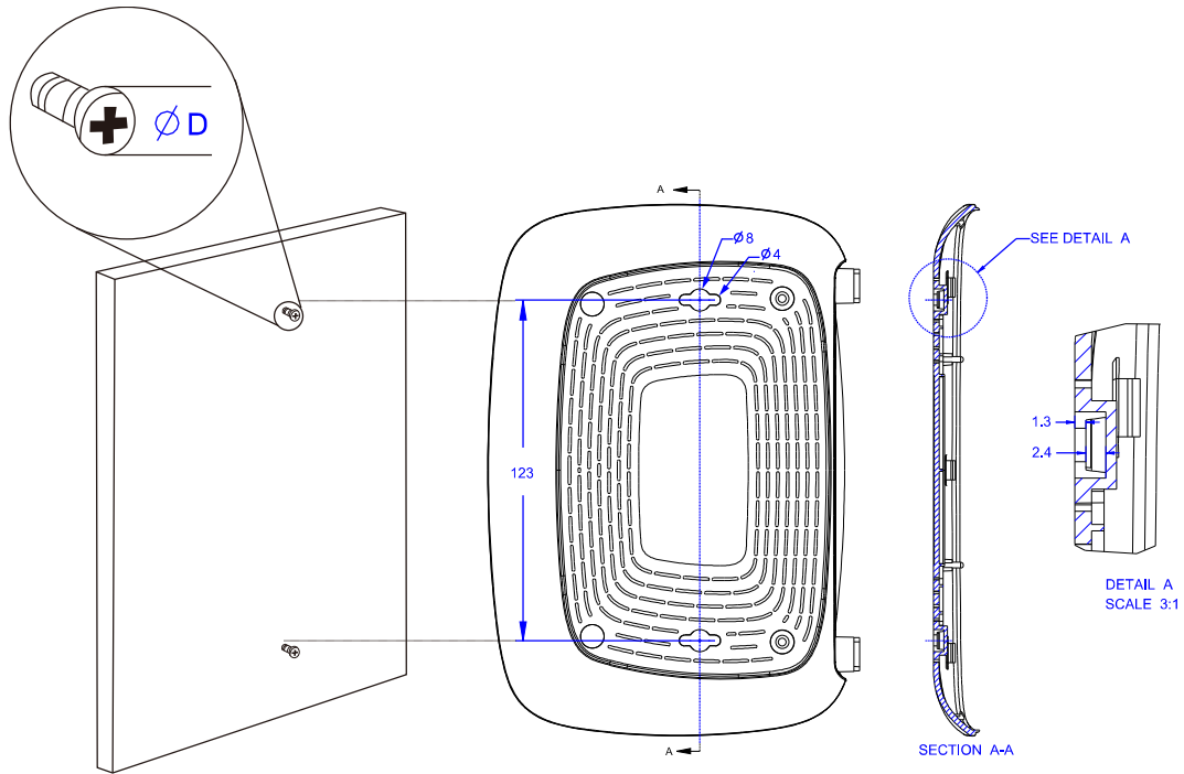
Figure 2-3 Wall-mount Install
