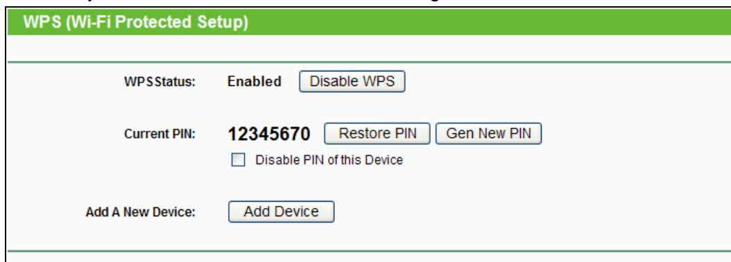
Figure 5-2 WPS
