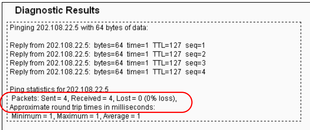
Figure 4-89 Diagnostic Results
