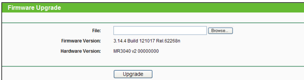
Figure 4-90 Firmware Upgrade
