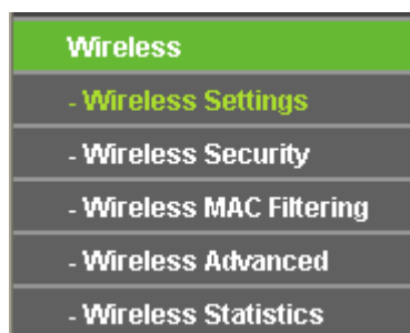
Figure 4-24 Wireless menu
