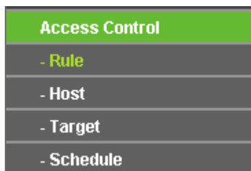
Figure 4-54 Access Control
