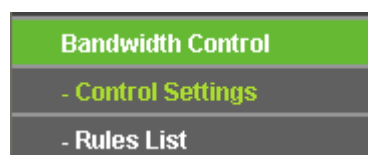
Figure 4-73 Bandwidth Control
