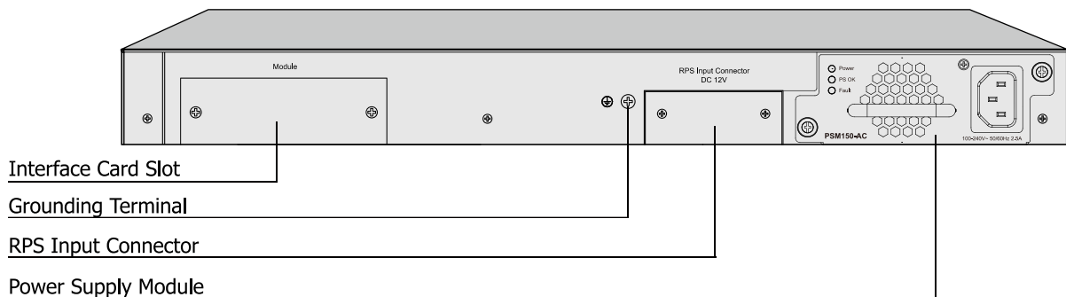
Figure 2-2 Rear Panel (1)
