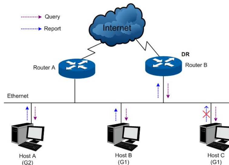
Figure 11-3 IGMP Query-and-Response
