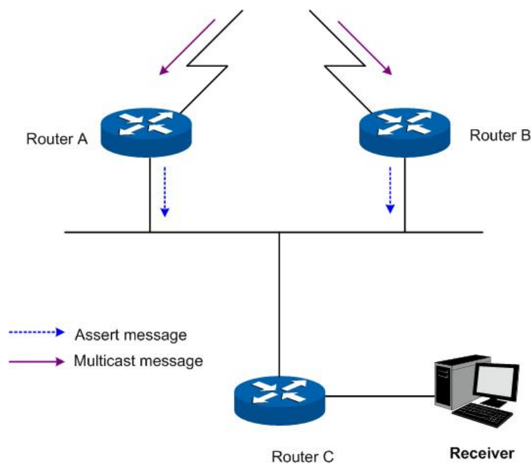
Figure 11-12 Assert Mechanism
