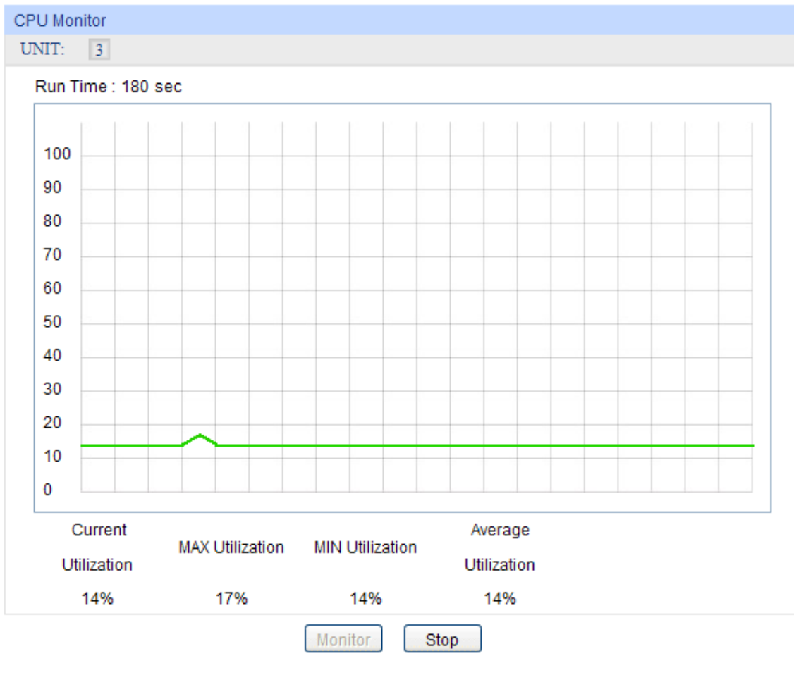
Figure18-1 CPU Monitor
