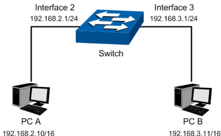
Figure 10-21 ARP Application
