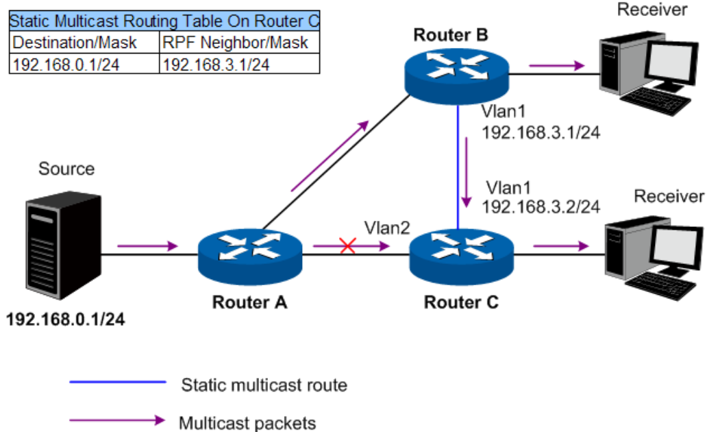
Figure 11-26 Static Multicast Routing
