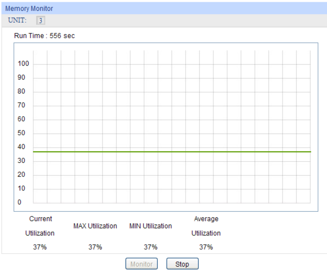
Figure18-2 Memory Monitor
