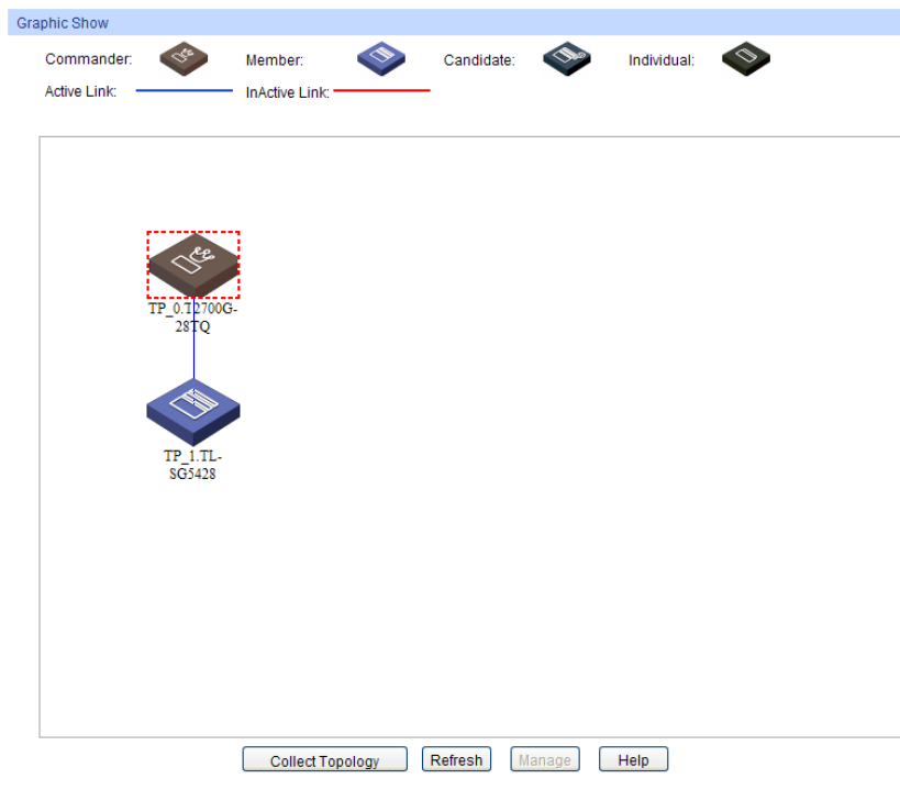
Figure17-18 Collect Topology
