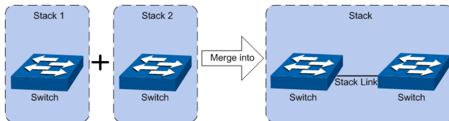
Figure 5-4 Stack Merge
