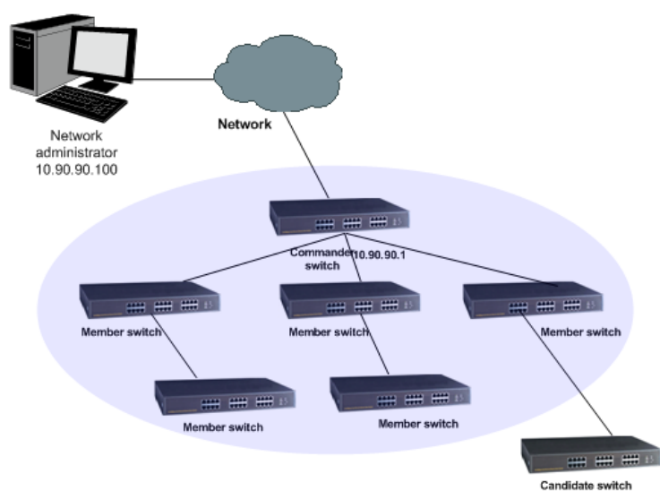
Figure17-1 Cluster topology
