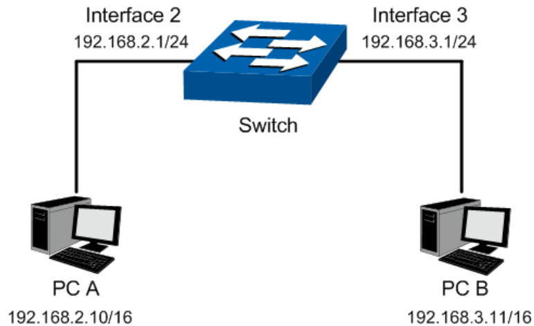
Figure 10-21 ARP Application
