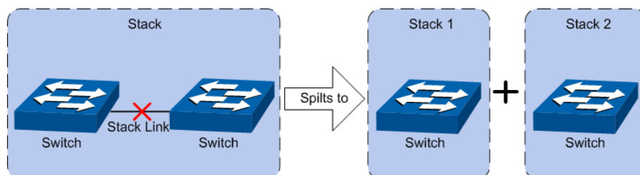
Figure 5-5 Stack Split
