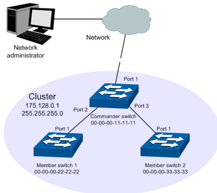
Figure17-19 Network diagram
