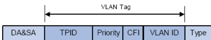
Figure 7-2 Format of VLAN Tag
