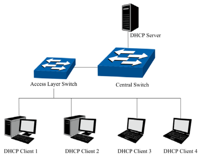
Figure 14-5 Network diagram for DHCP-snooping implementation
