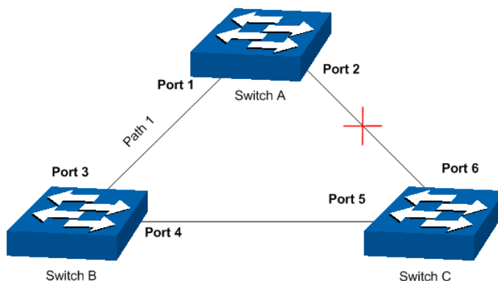
Figure 8-1 Basic STP diagram
