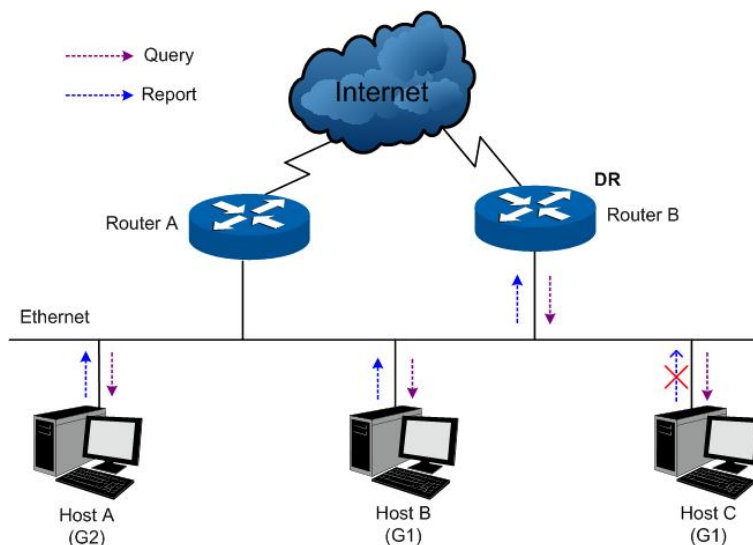
Figure 11-3 IGMP Query-and-Response
