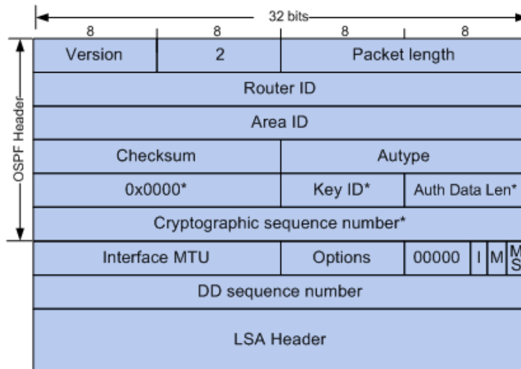
Figure 10-41 DD Packet
