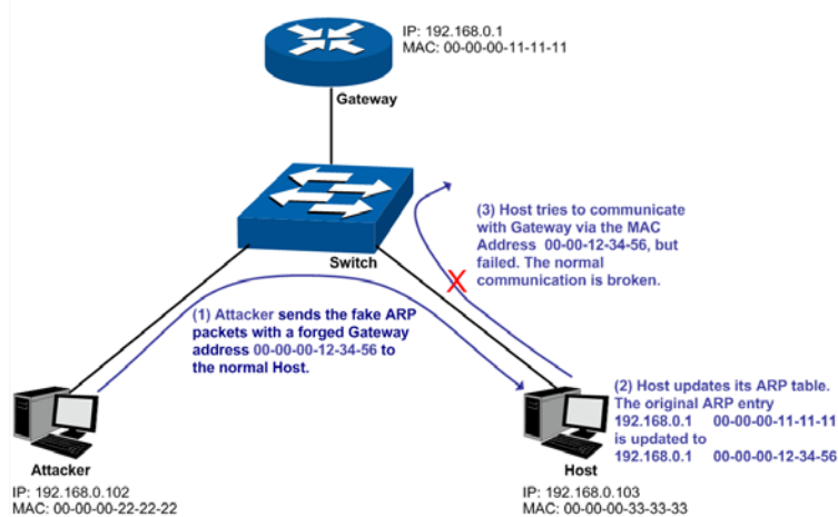
Figure 14-10 ARP Attack - Imitating Gateway
