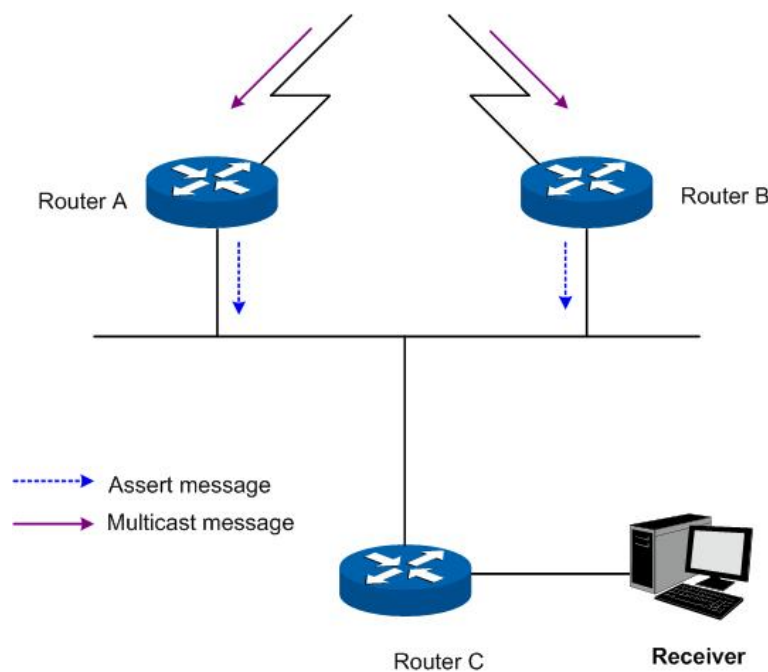
Figure 11-12 Assert Mechanism
