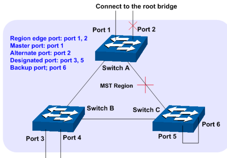
Figure 8-3 Port roles
