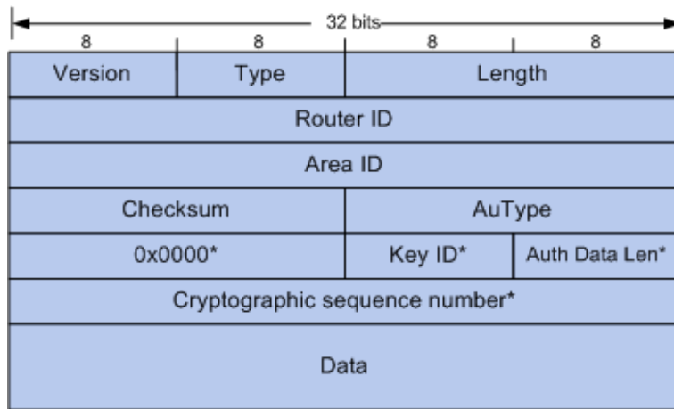
Figure 10-39 OSPF Header
