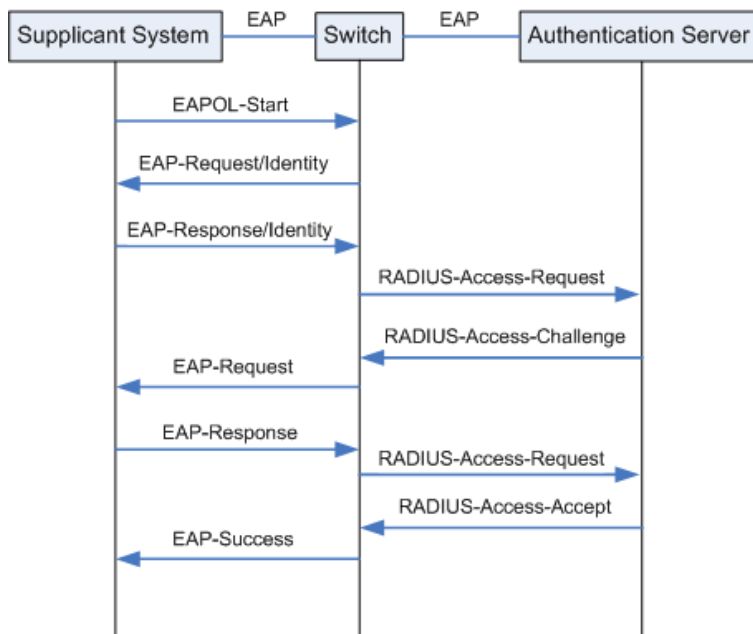
Figure 14-20 EAP-MD5 Authentication Procedure
