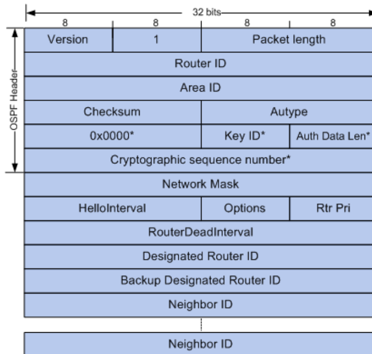
Figure 10-40 HELLO Packet
