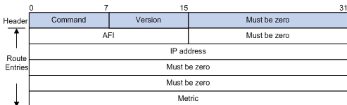
Figure 10-24 RIPv1 Message Format
