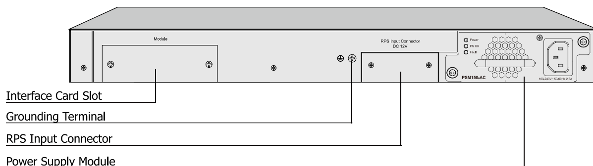
Figure 2-2 Rear Panel (1)
