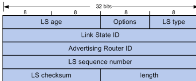
Figure 10-44 LSA Header
