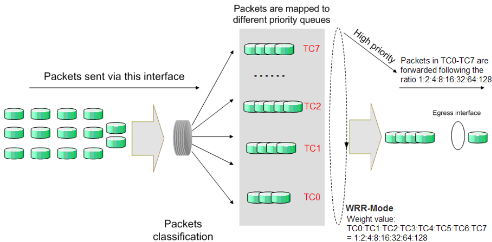
Figure 12-5 WRR-Mode
