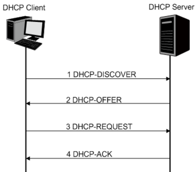
Figure 14-6 Interaction between a DHCP client and a DHCP server
