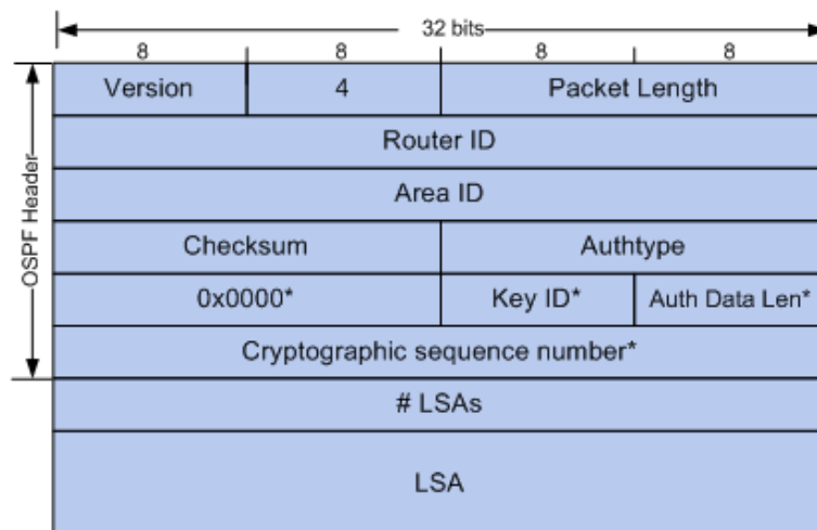
Figure 10-43 LSU Packet
