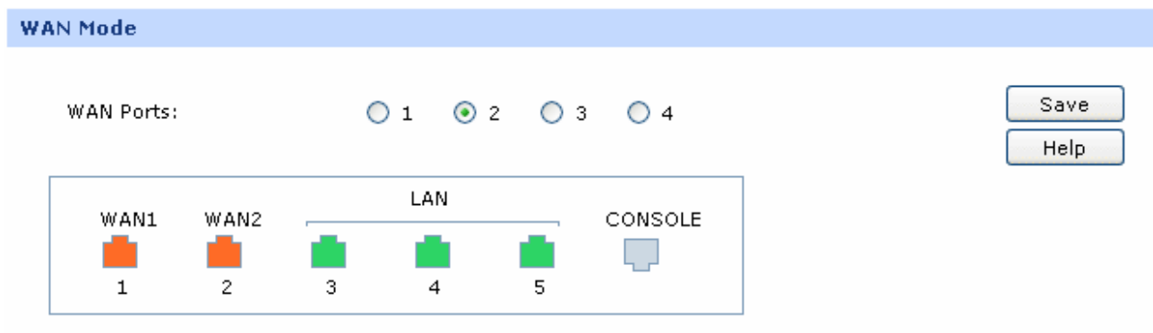
Figure 4-2 WAN Mode
