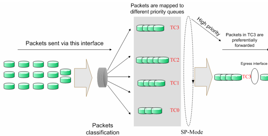
Figure 9-4 SP-Mode
