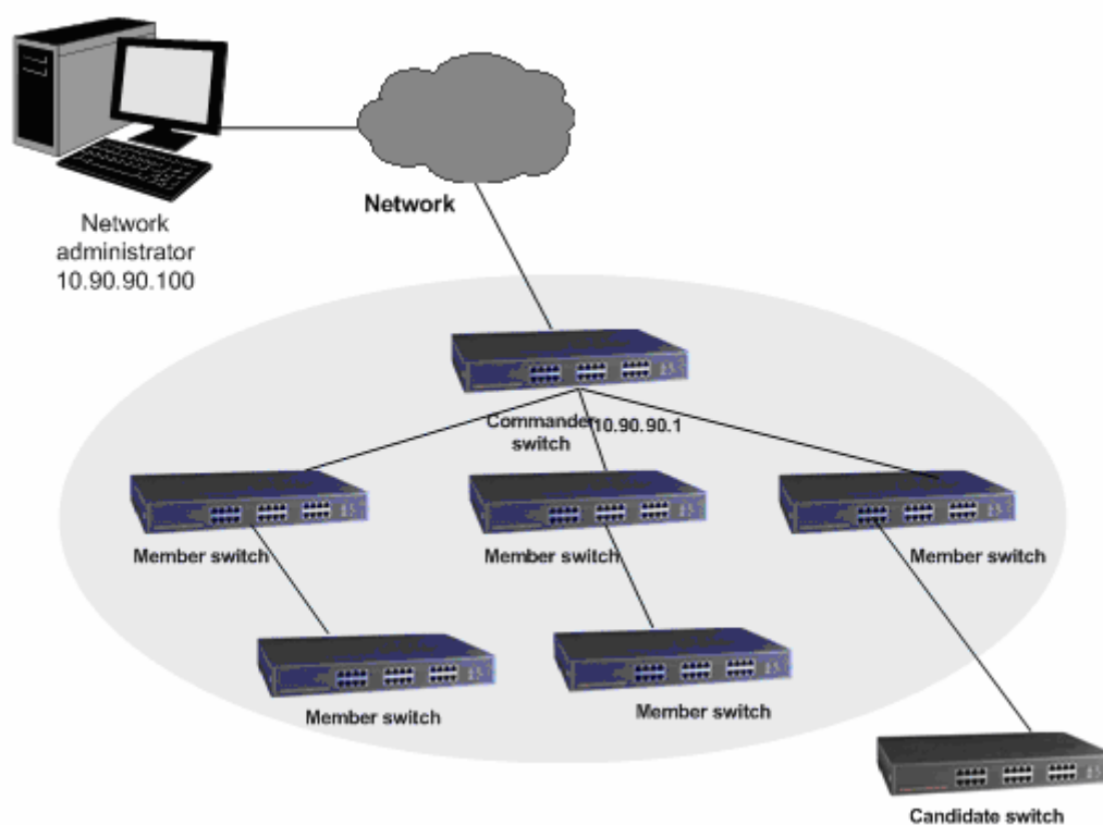
Figure 14-1 Cluster topology
