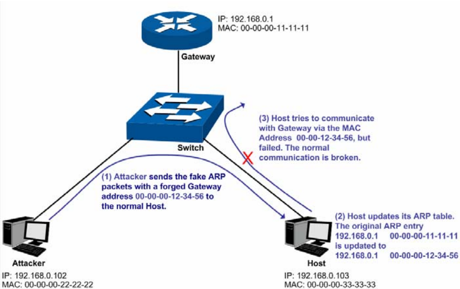
Figure 11-9 ARP Attack - Imitating Gateway
