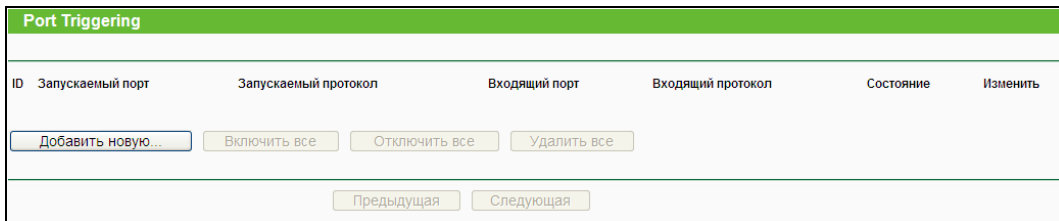
Рис. 4-32 Port Triggering
