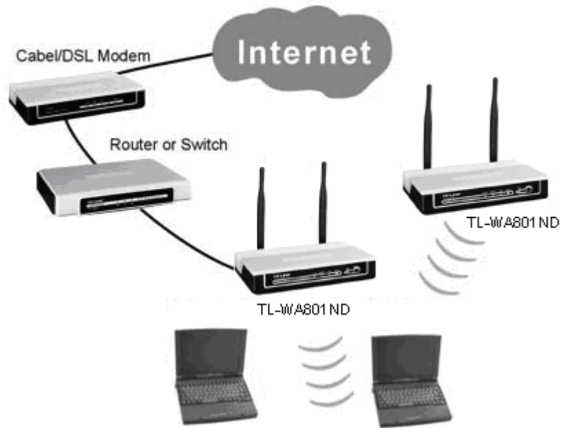
Figure 2-1 The Example of Infrastructure Network Incorporating the TL-WA801ND
