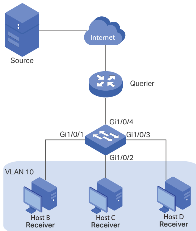
Figure 7-19 Network Topology for Multicast Filtering
