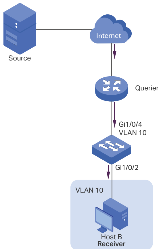
Figure 7-15 Network Topology for Unknown Multicast and Fast Leave
