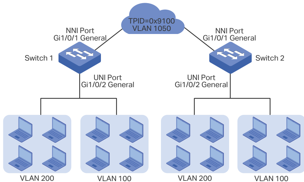
Figure 4-1 Network Topology
