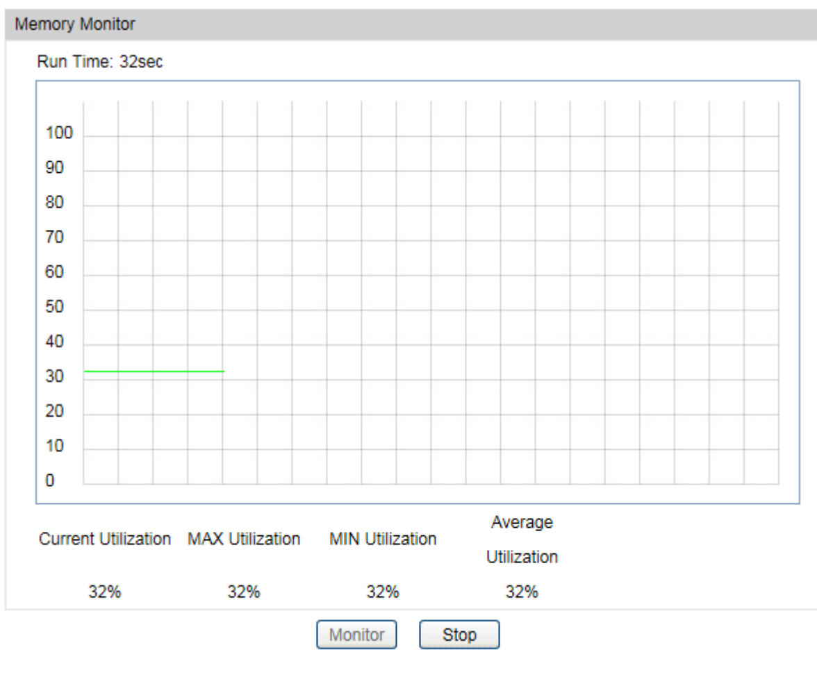
Figure 15-2 Memory Monitor
