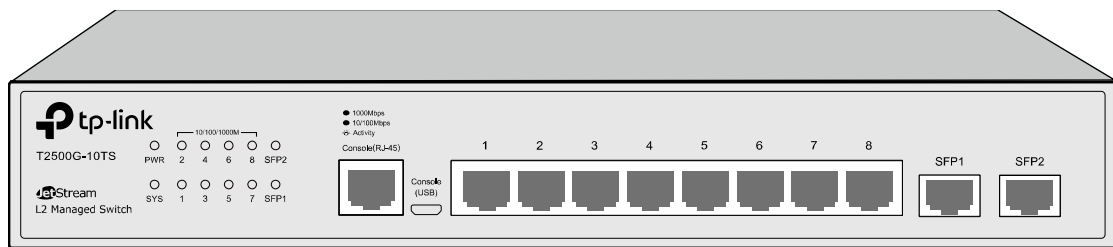
Figure 2-1 Front Panel
