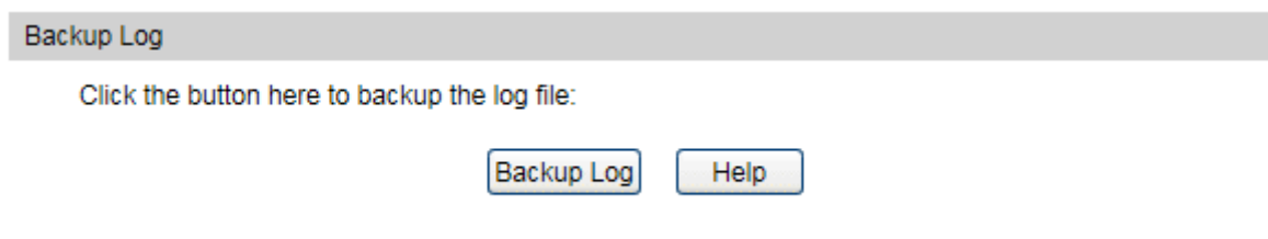
Figure 15-6 Backup Log
