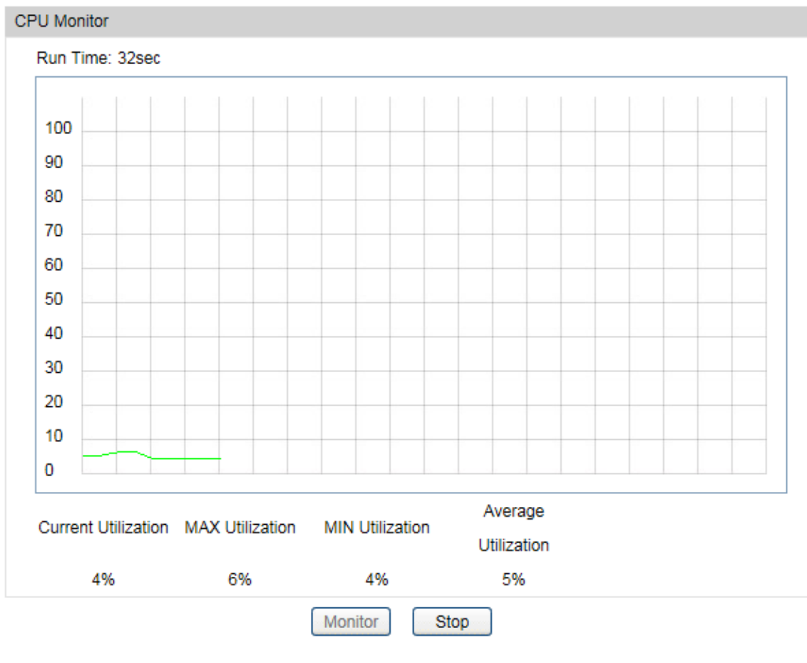
Figure 15-1 CPU Monitor
