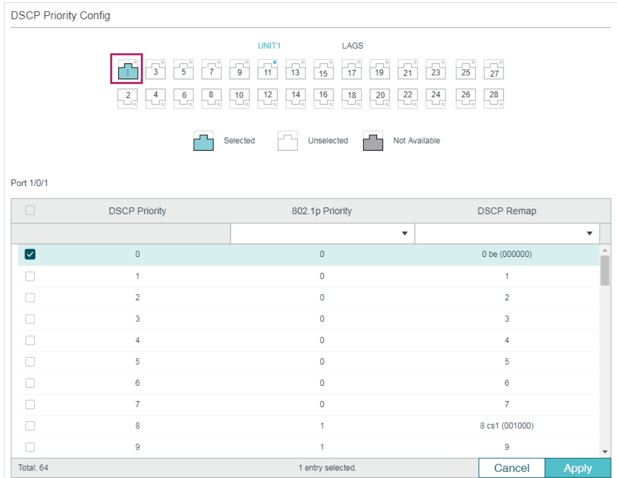
Figure 2-8 Configuring the DSCP to 802.1p Mapping and the DSCP Remap
