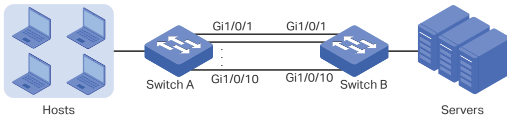
Figure 3-4 Network Topology
