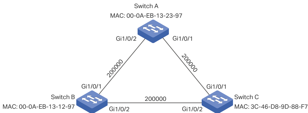
Figure 5-1 Network Topology
