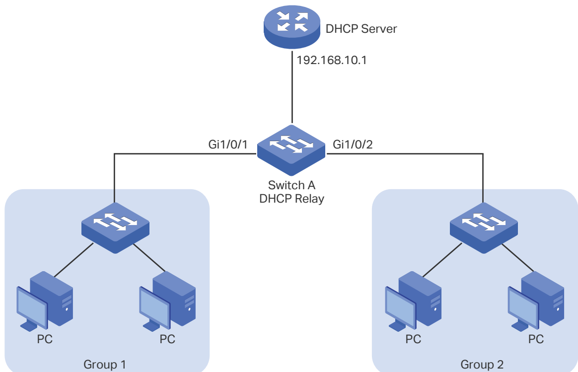
Figure 5-28 Network Topology for DHCP L2 Relay
