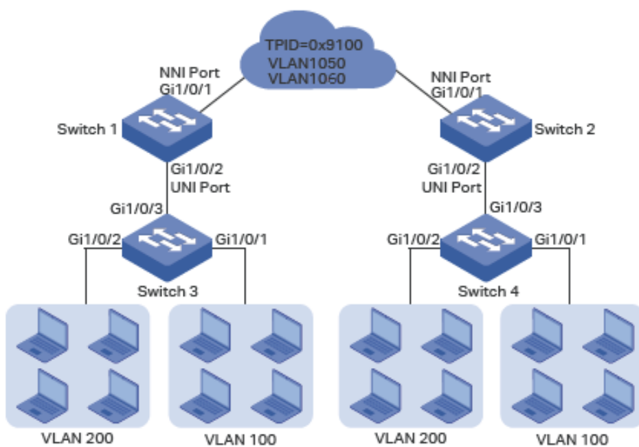
Figure 4-10 Network Topology
