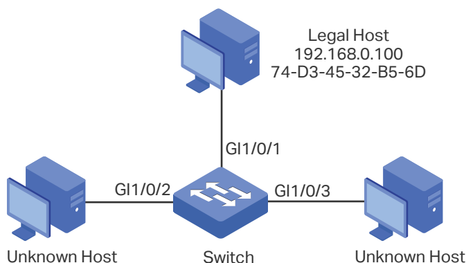
Figure 5-6 Network Topology
