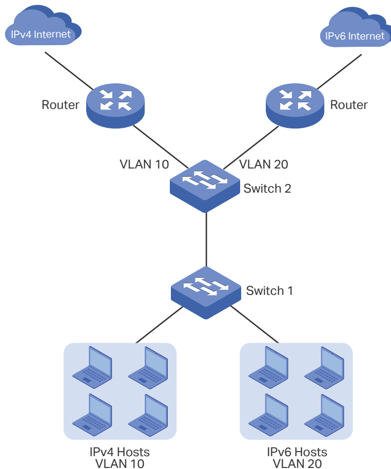
Figure 1-1 Common Application Scenario of Protocol VLAN
