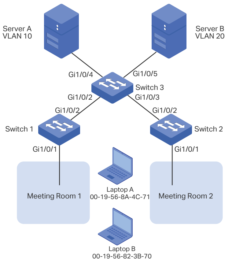
Figure 3-1 Network Topology
