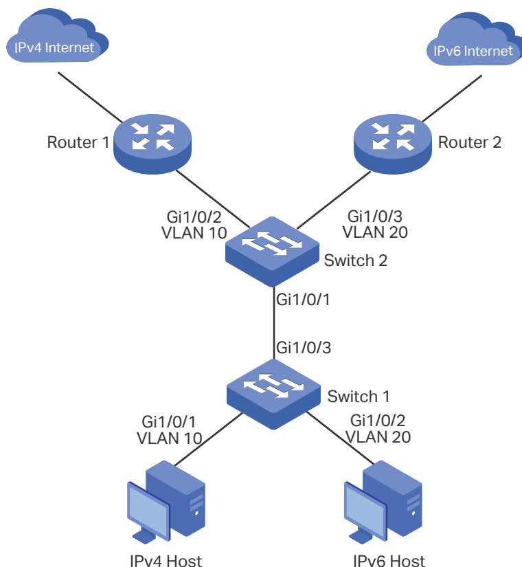
Figure 3-1 Network Topology
