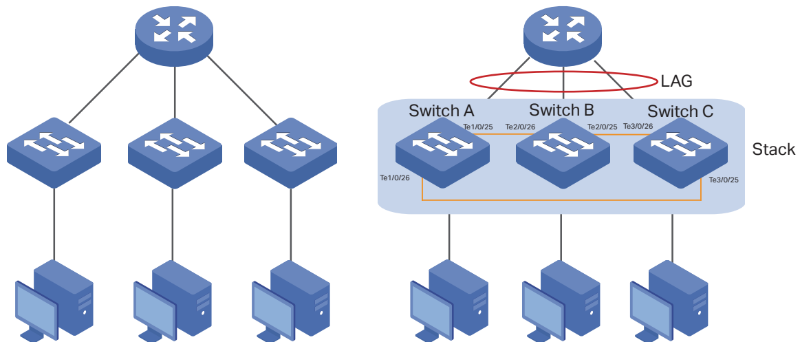
Figure 3-1 Network Topology
