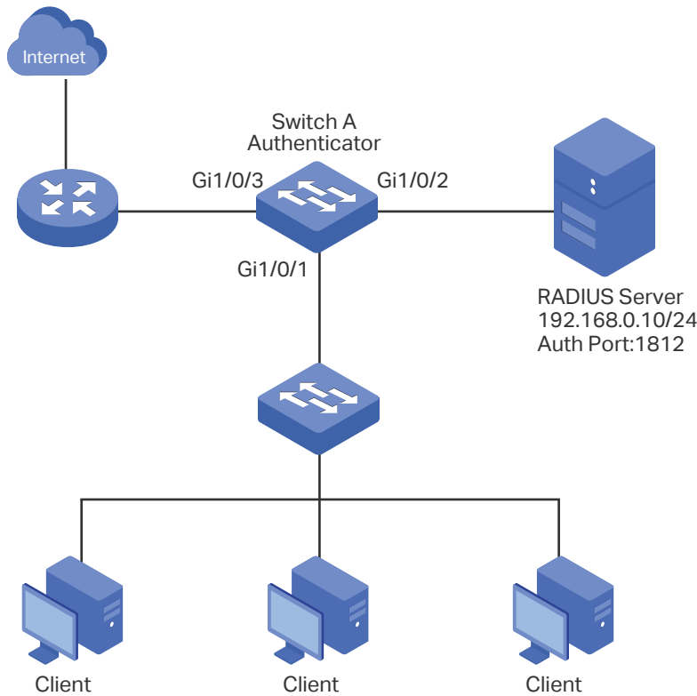
Figure 3-1 Network Topology
