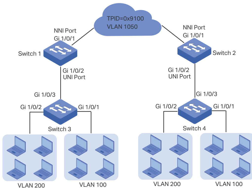
Figure 4-1 Network Topology
