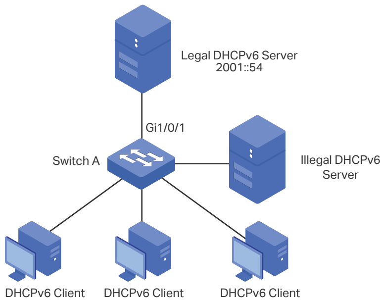
Figure 4-1 Network Topology
