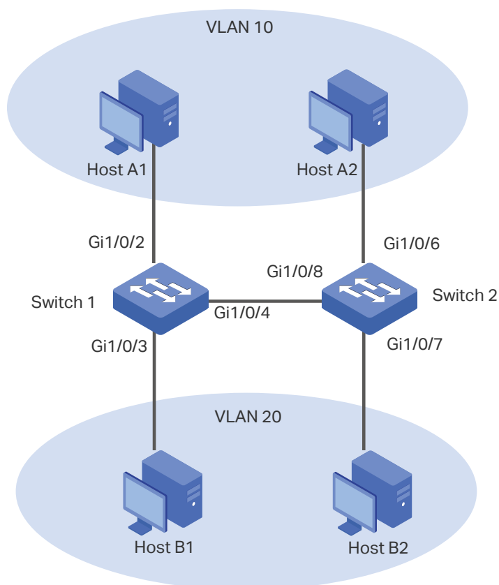
Figure 3-1 Network Topology
