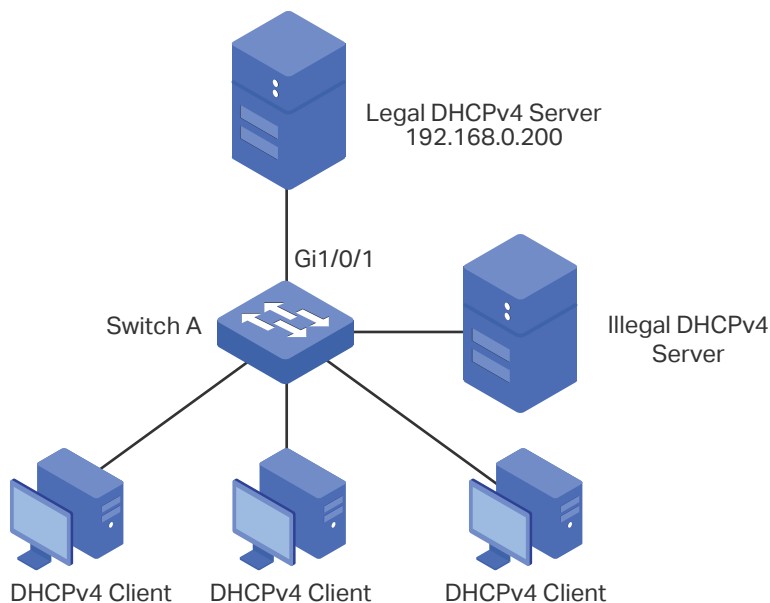
Figure 4-1 Network Topology
