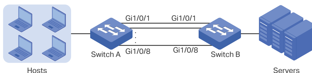
Figure 3-1 Network Topology
