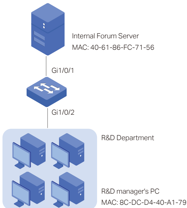
Figure 3-1 Network Topology
