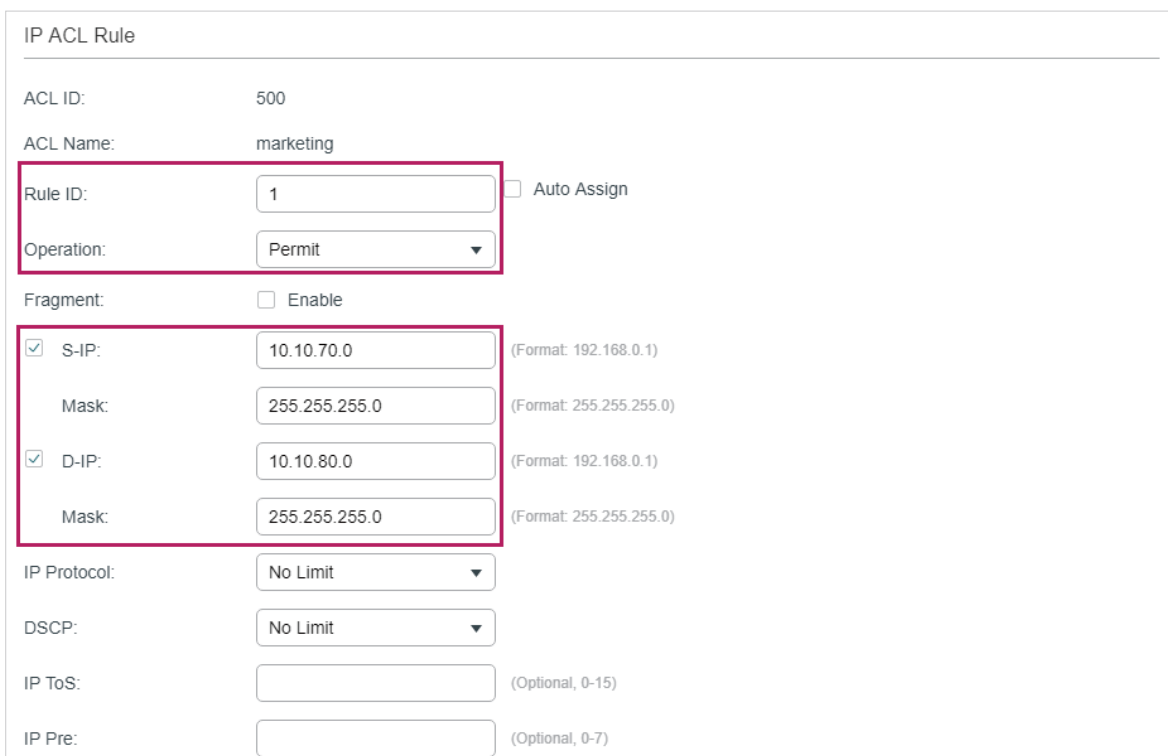
Figure 3-16 Configuring Rule 1
