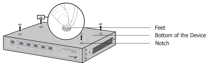
Figure 2-1 Desktop Installation
