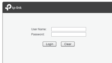
Figure 5-3 Login
