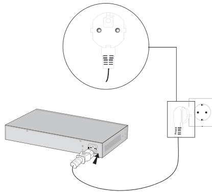
Figure 3-1 Connecting to the Ground
