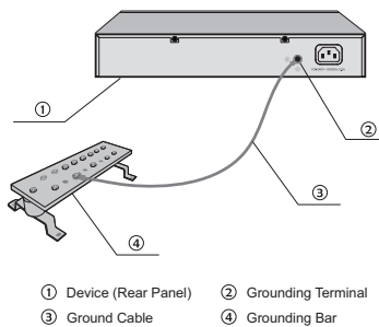
Figure 3-2 Connecting to the Grounding Bar
