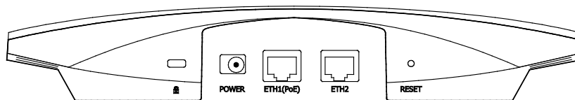
Figure 1-3 Interface Panel of EAP330
