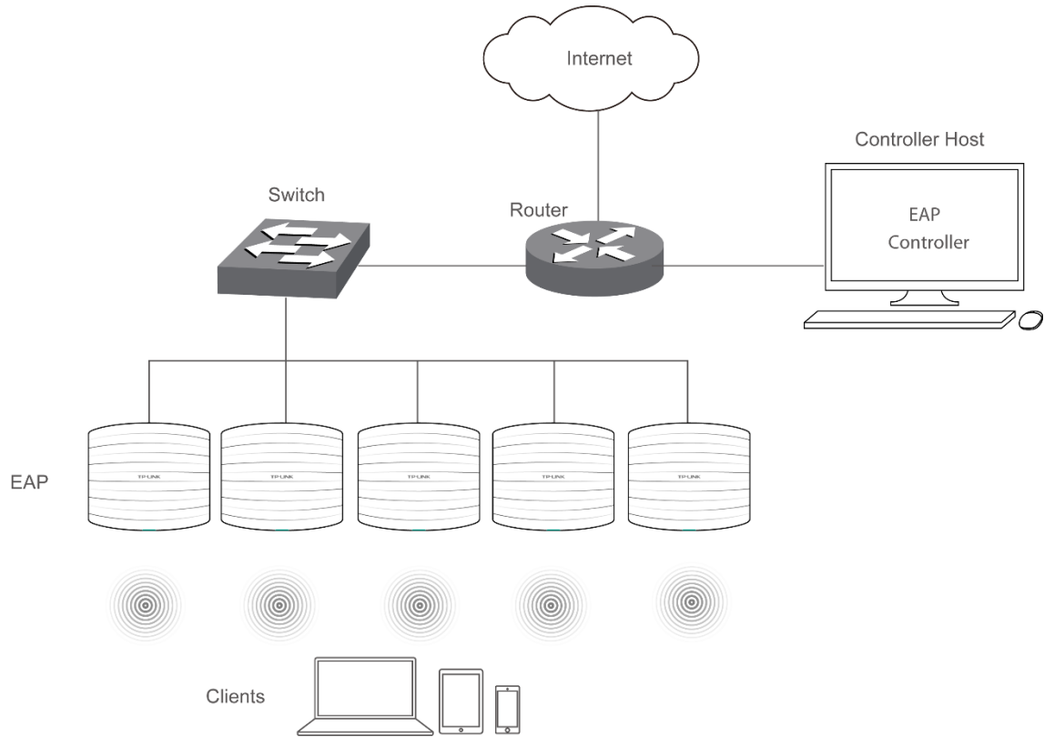
Figure 2-1 Typical Topology
