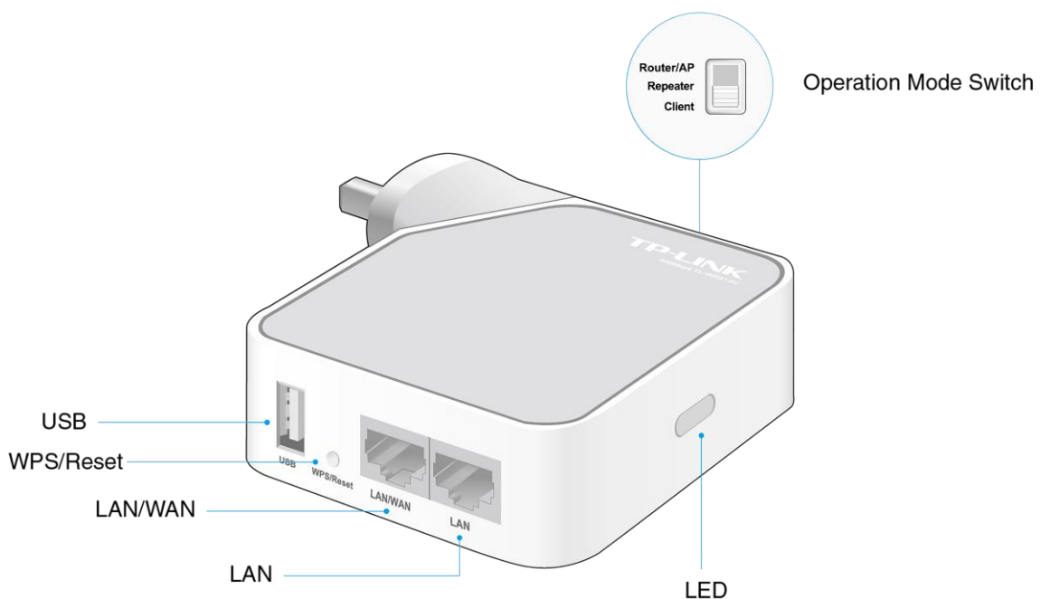
Figure 1-1 TL-WR810N sketch
