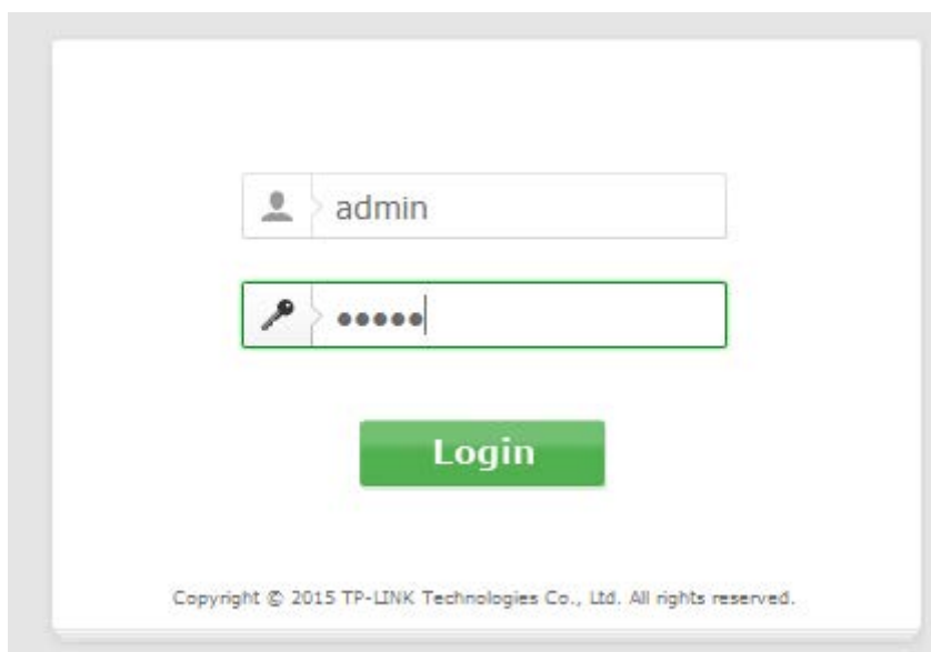
Figure 3-4 Login Windows
