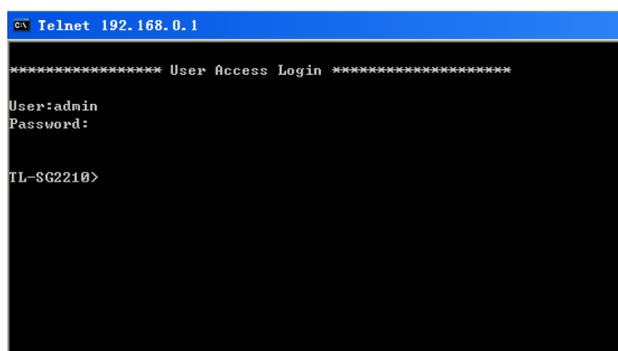
Figure 1-4 Log in the Switch
