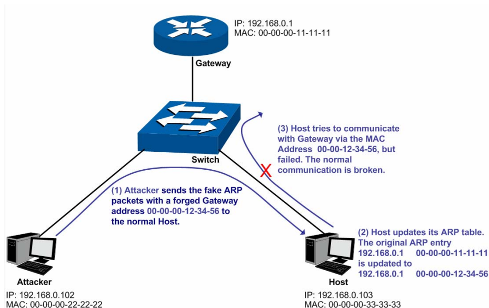
Figure 12-9 ARP Attack - Imitating Gateway
