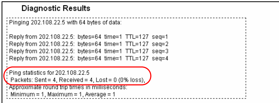
Figure 7-27 Diagnostic Results
