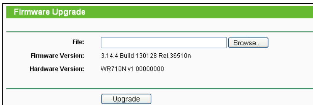
Figure 8-88 Firmware Upgrade
