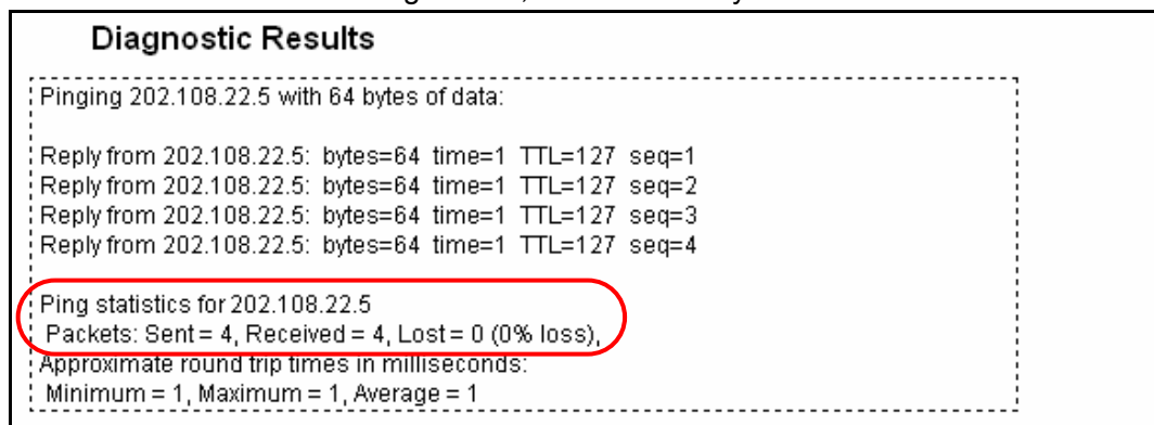
Figure 6-32 Diagnostic Results
