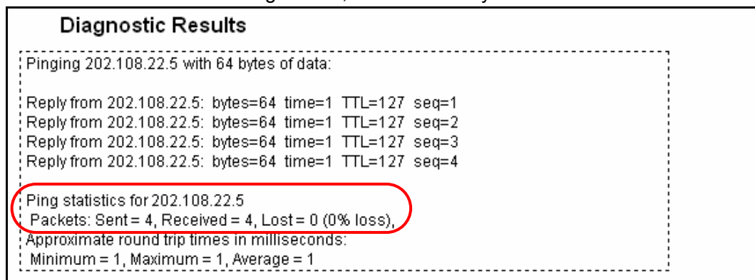
Figure 5-35 Diagnostic Results
