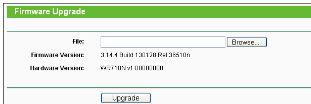
Figure 5-36 Firmware Upgrade
