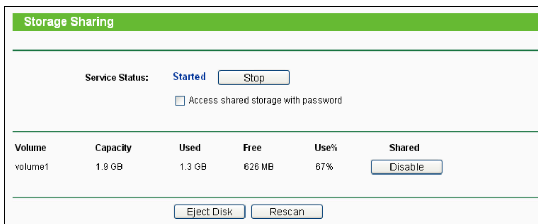
Figure 4-34 Storage Sharing
