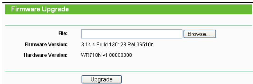
Figure 7-28 Firmware Upgrade
