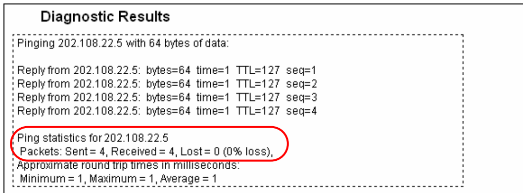
Figure 8-87 Diagnostic Results
