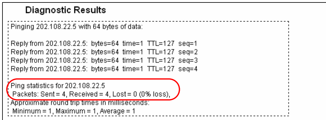
Figure 4-91 Diagnostic Results
