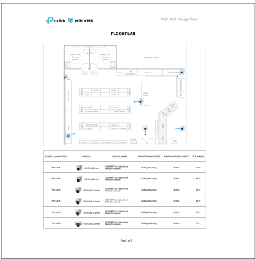
Floor Plan
