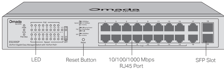
Figure 1-4 Front Panel of ES220GP
