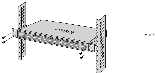
Figure 2-3 Rack Installation
