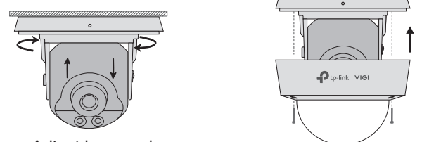
Reinstall the top cover
